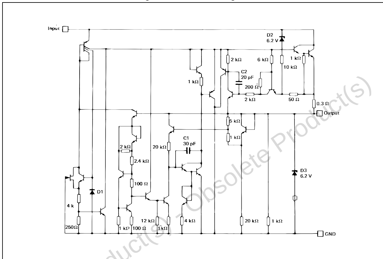
Figure 1. Schematic diagram
