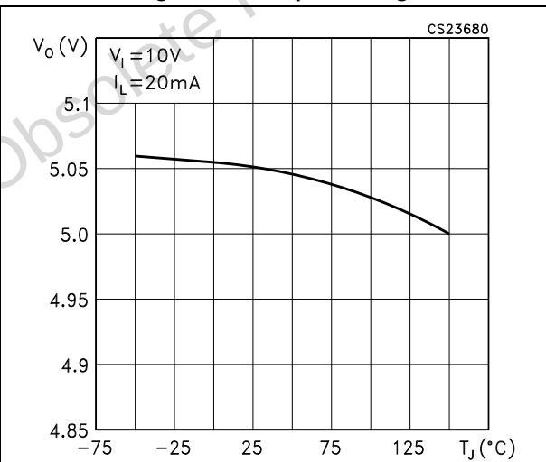
Figure 10. Output voltage
