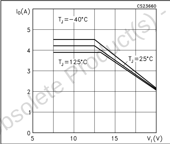
Figure 5. Peak available output current
