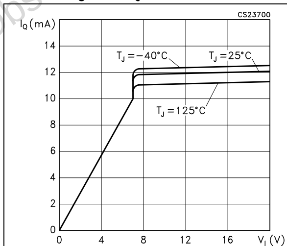
Figure 11. Quiescent current
