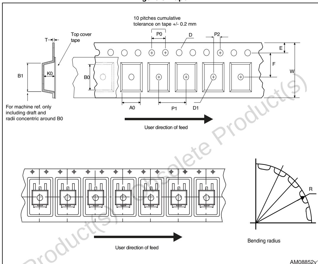
Figure 8. Tape
