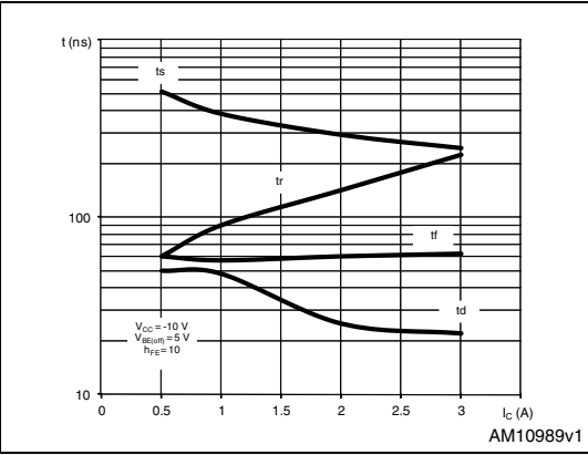
Figure 8. Resistive load switching times
