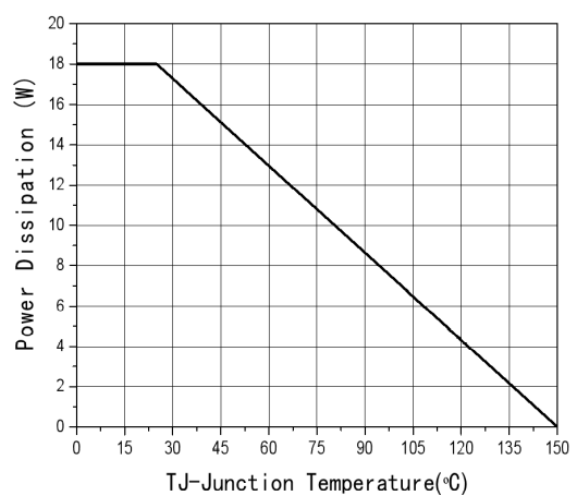
Fig8 Power De-rating
