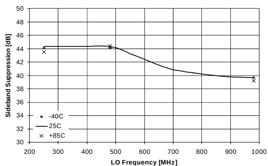
Sideband Suppression vs. LO Frequency
