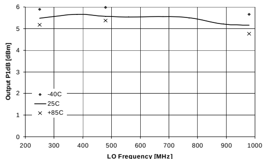
Output P1dB vs. LO Frequency
