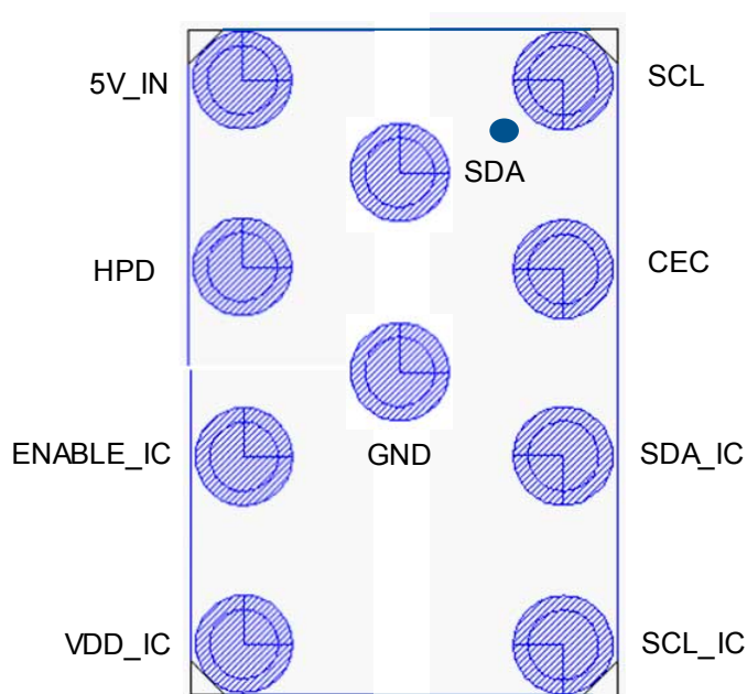
Figure 1. Pin configuration (bump side)
