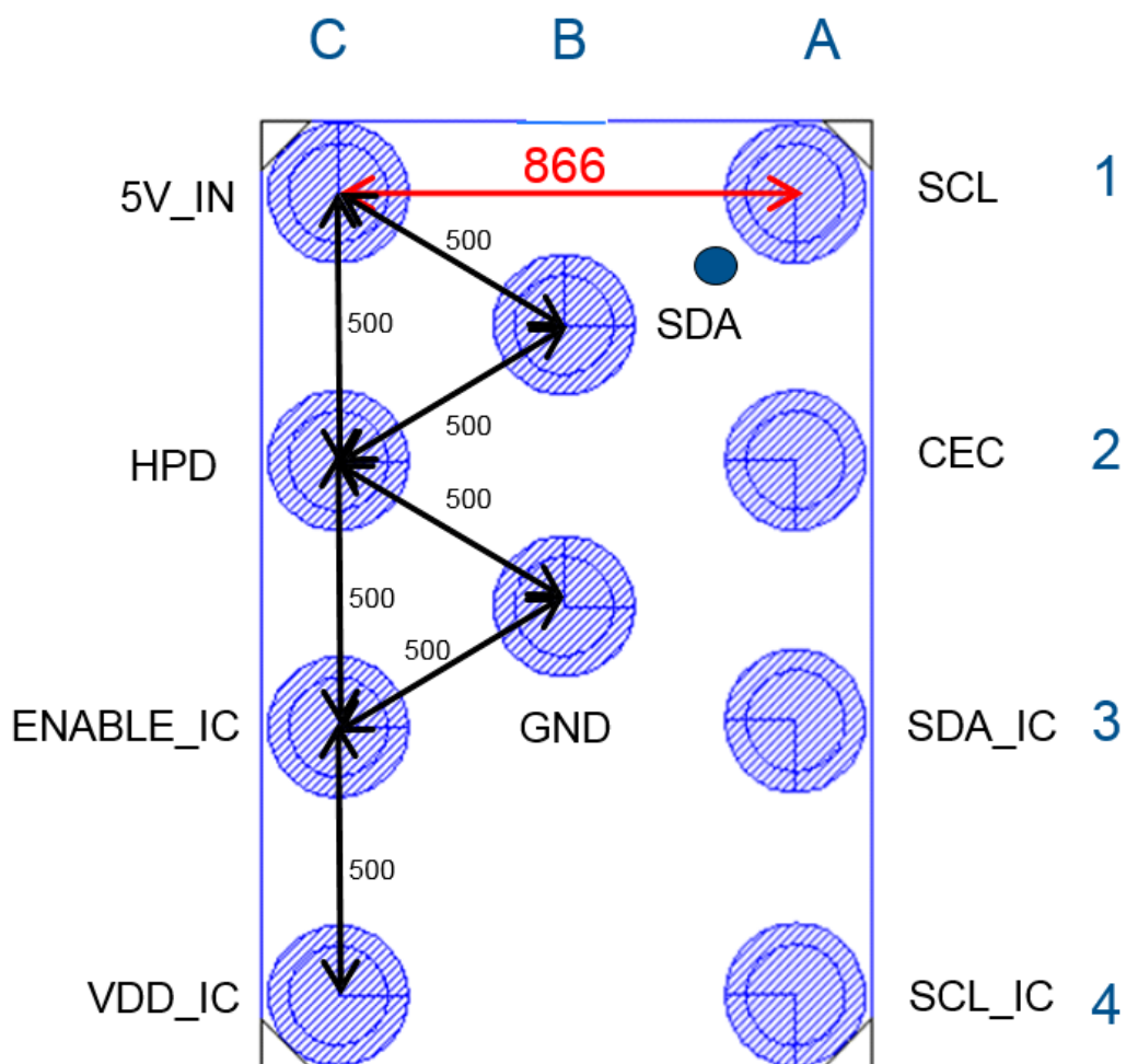
Figure 7. Pin numbering (bump side)
