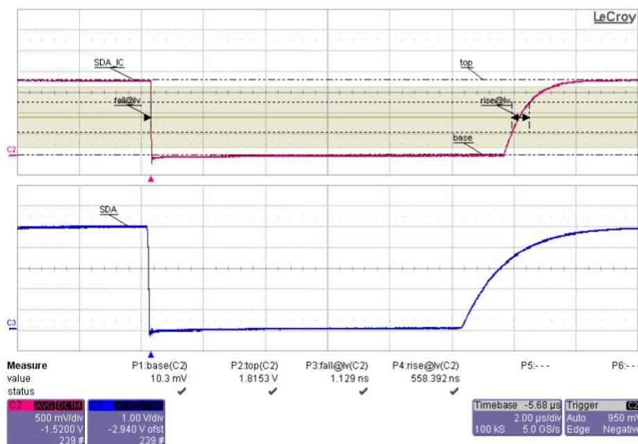
Figure 9. DDC typical waveforms - communication from source to sink
