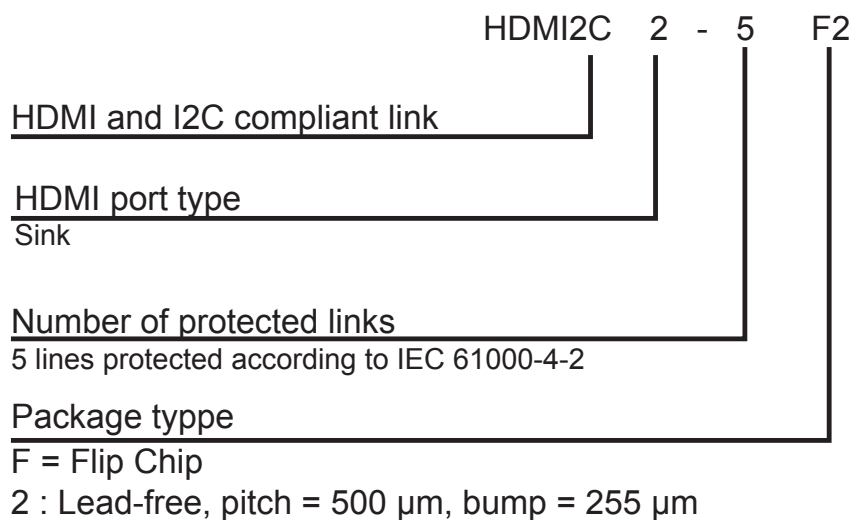
Figure 14. Ordering information scheme
