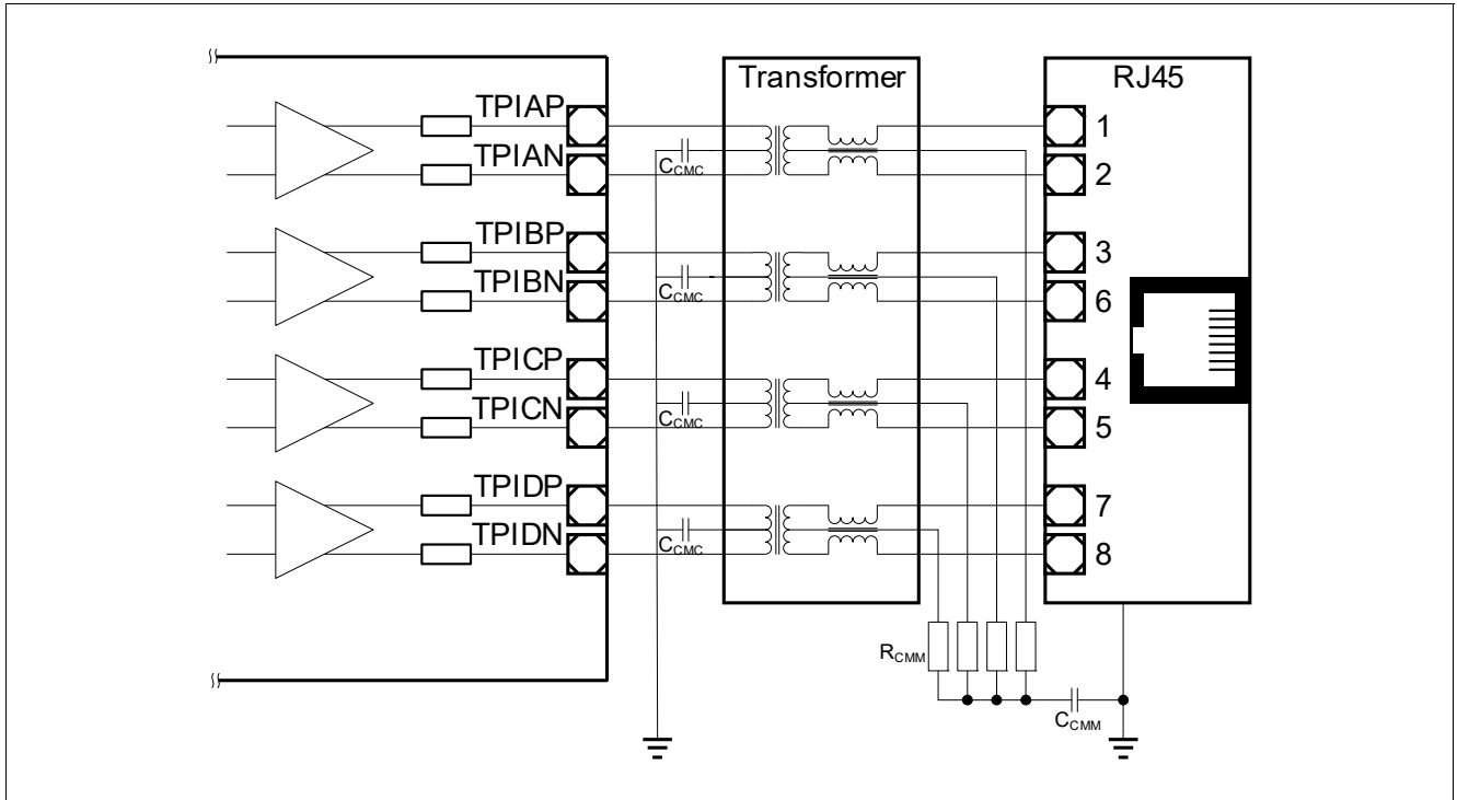
Figure 5 Twisted-Pair Interface of GPY211 Including Transformer and RJ45 Plug
