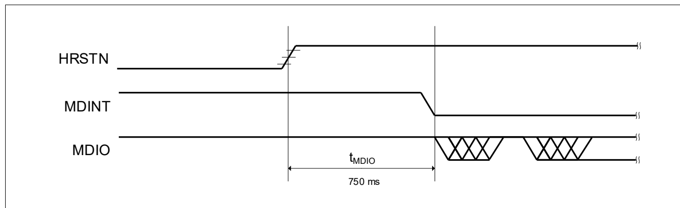
Figure 4 MDIO Access Timing
