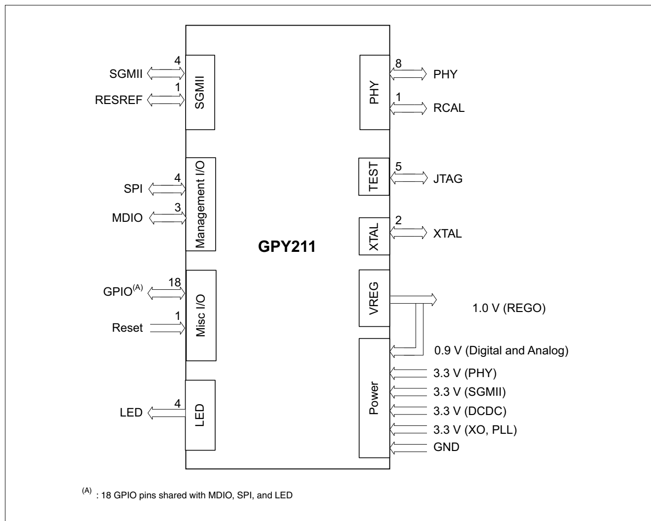
Figure 2 GPY211 External Signals Overview
