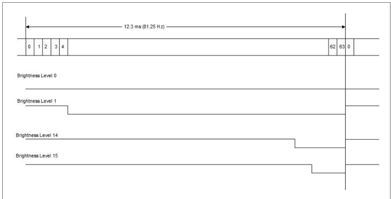
Figure 13 LED Brightness Control By Controlling LED Output Enable/Disable
