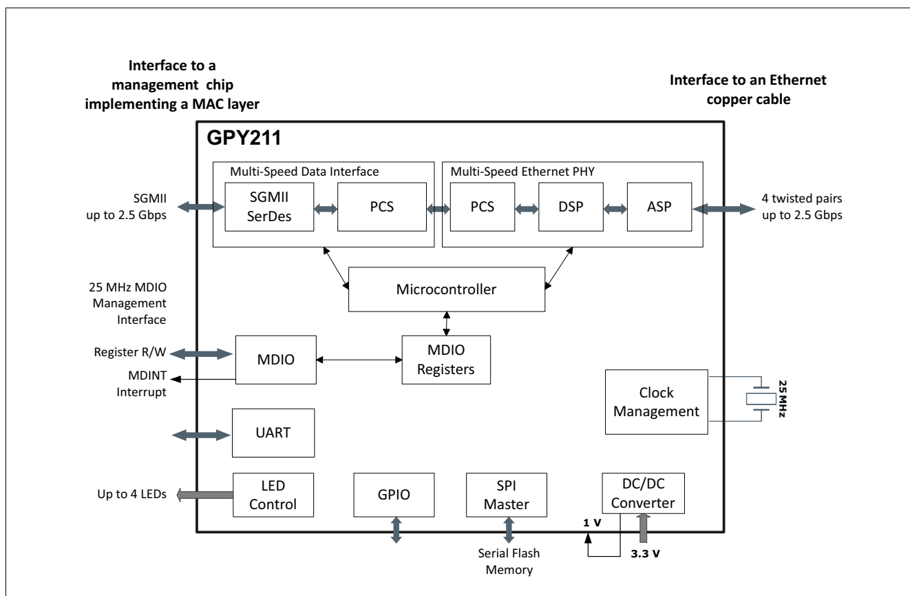
Figure 1 GPY211 Block Diagram
