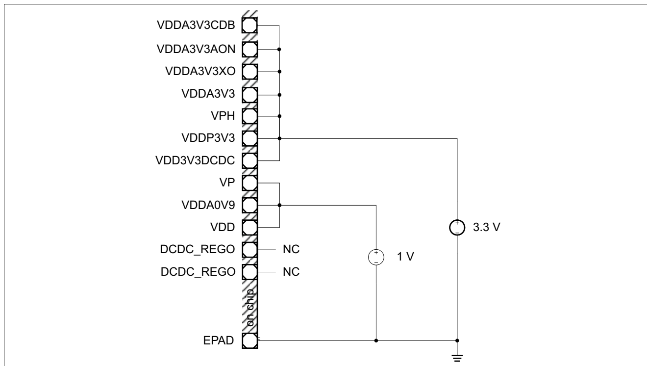
Figure 29 External Circuitry without using the Integrated DC/DC Converter
