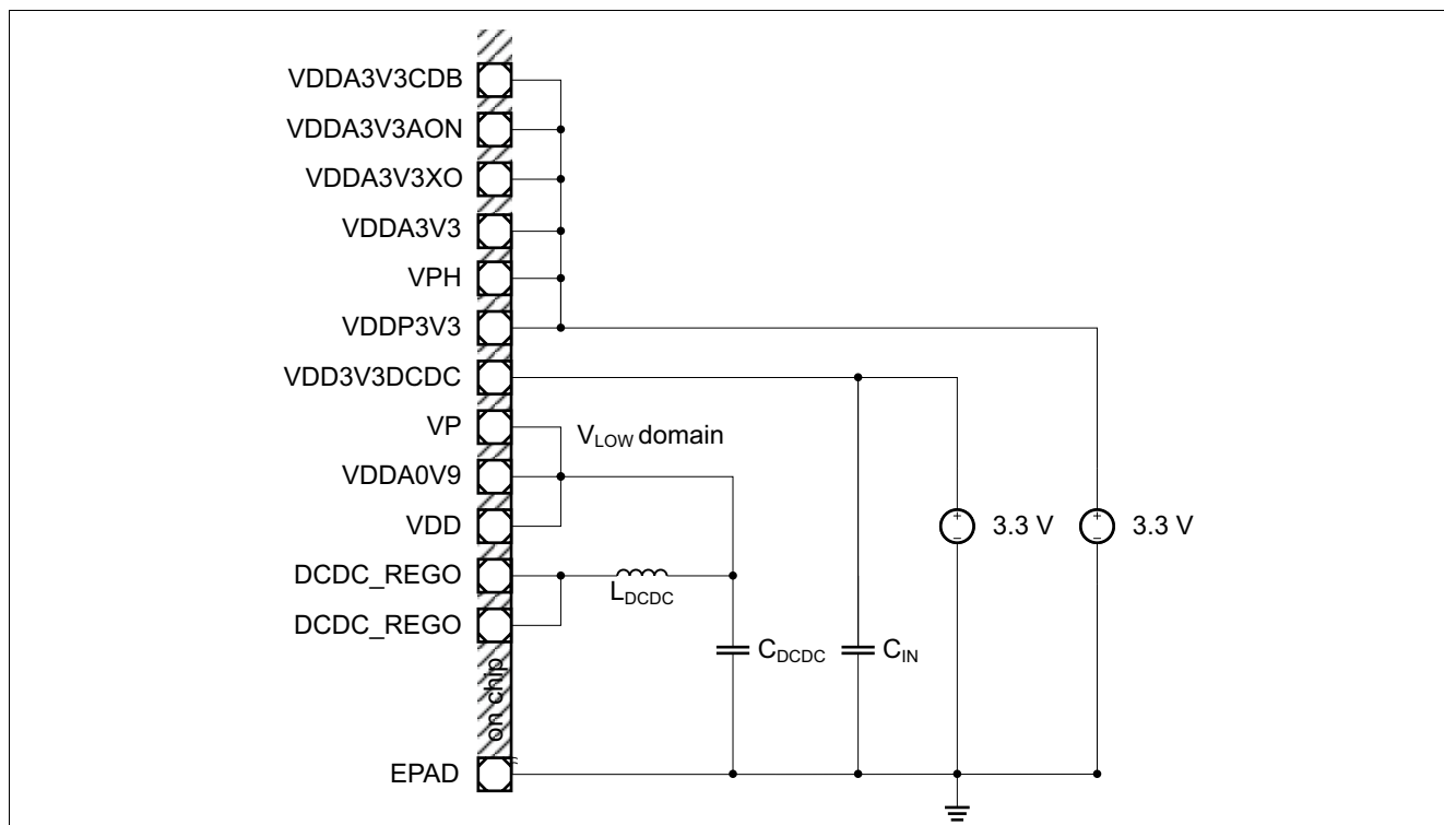
Figure 28 External Circuitry Using the Integrated DC/DC Converter
