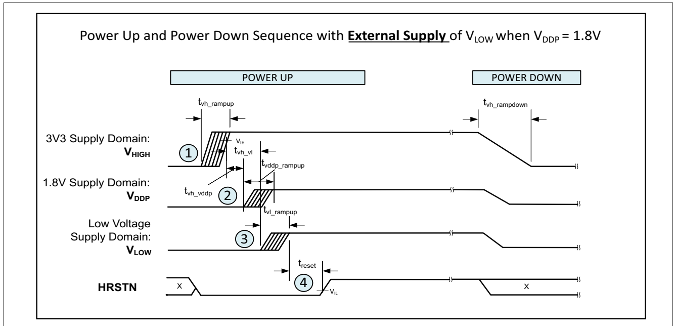
Figure 18 Timing Diagram for the Reset Sequence (External supply of V_{LOW} domain) when V_{DDP}=1.8 V
