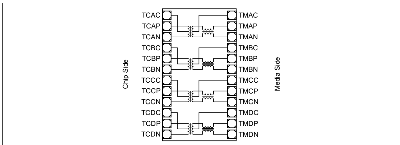
Figure 27 Schematic of an Ethernet Transformer Device
