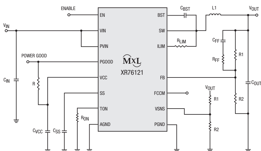
Figure 1. Typical Application
