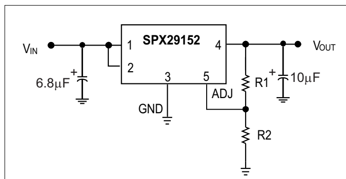
Figure 2: Adjustable Output Linear Regulator
