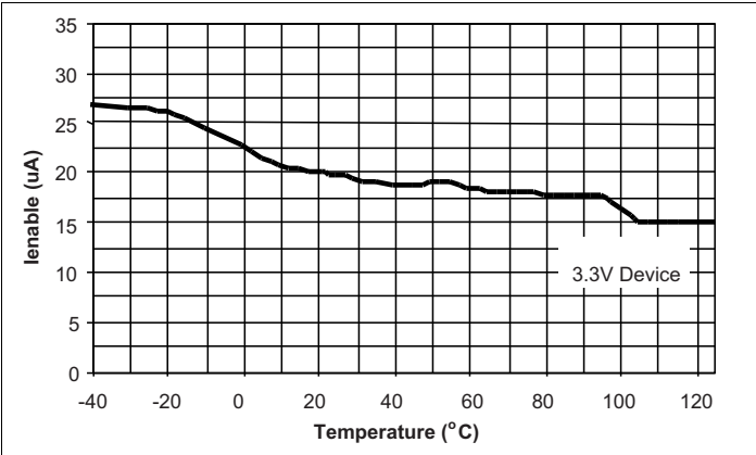
Figure 22: ENABLE Current vs Temperature at V_{EN} = 16V
