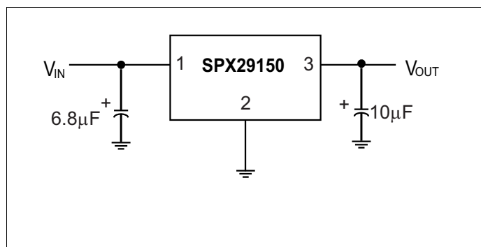
Figure 1: Fixed Output Linear Regulator
