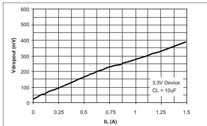
Figure 13: Dropout Voltage vs Load Current
