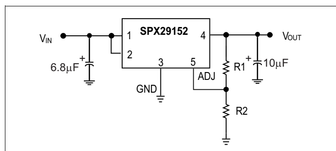
Figure 7: Adjustable Output Linear Regulator
