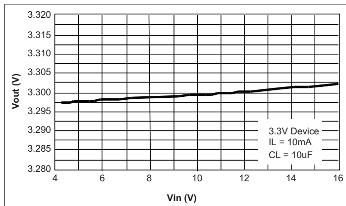
Figure 8: Line Regulation
