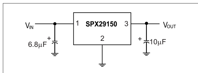
Figure 6: Fixed Output Linear Regulator
