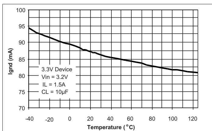
Figure 19: Ground Current vs Temperature in Dropout
