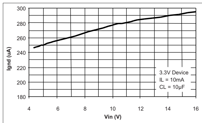
Figure 11: Ground Current vs Input Voltage
