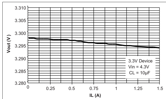
Figure 9: Load Regulation
