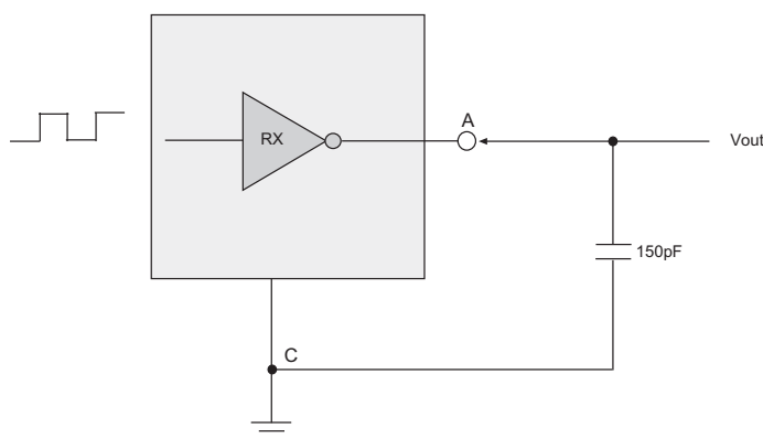
Figure 6: Receiver Propagation Delay and Transition Time Test Circuit
