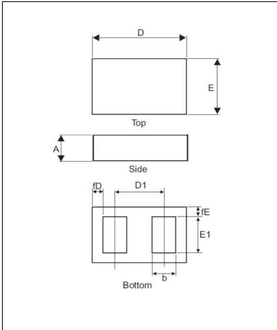
Figure 9: 0201 package outline
