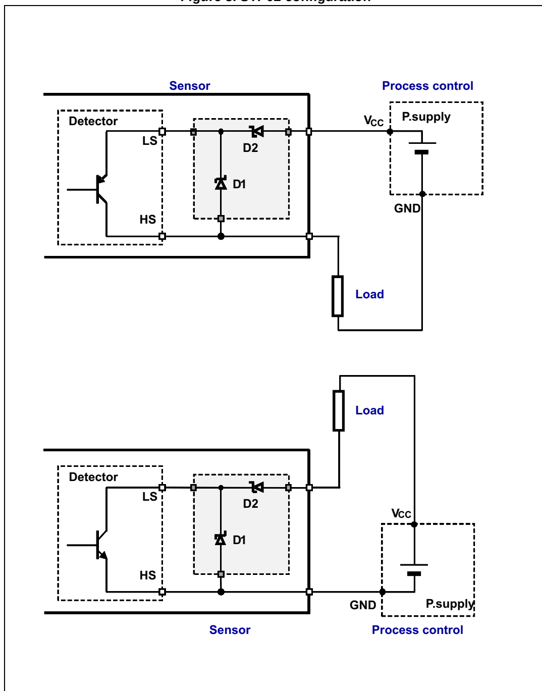
Figure 3. STP02 configuration
