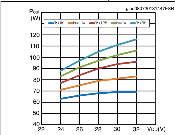
Figure 9. Output power vs supply voltage, freq = 945 MHz, I_{dq} = 0.4\text{ A}
