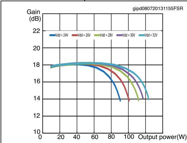
Figure 7. Gain vs output power, freq = 945 MHz, I_{dq} = 0.4\text{ A}
