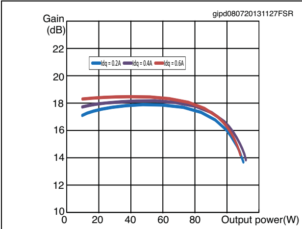
Figure 5. Gain vs output power, freq = 945 MHz, V_{dd} = 28 V
