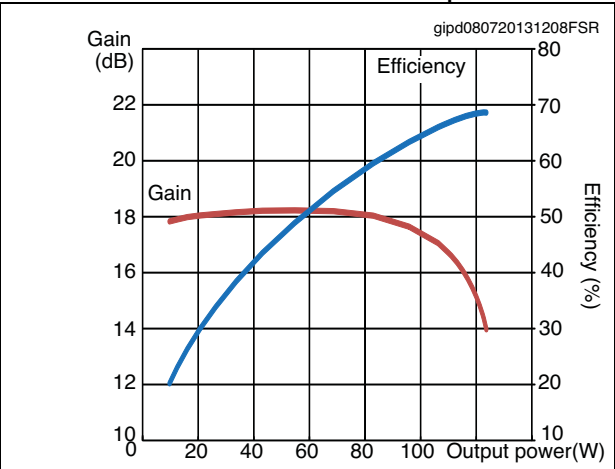
Figure 8. Gain and efficiency vs output power, freq = 945 MHz, V_{dd} = 32\text{ V} , I_{dq} = 0.4\text{ A}
