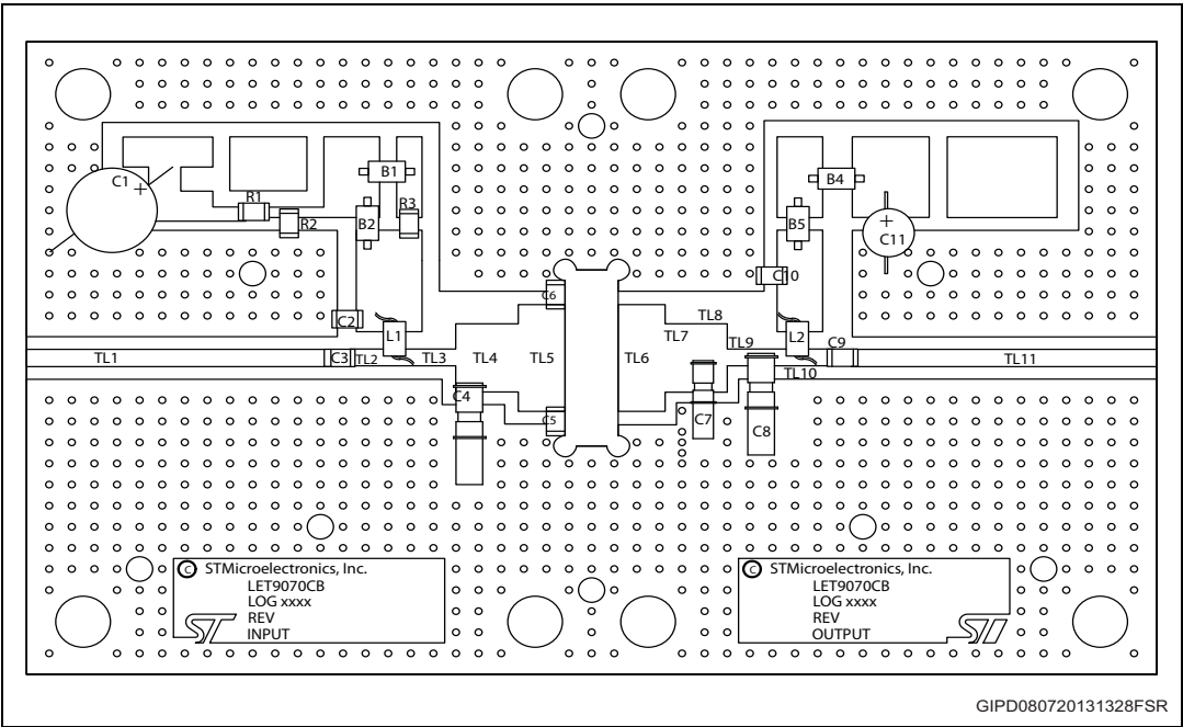
Figure 11. Test circuit
