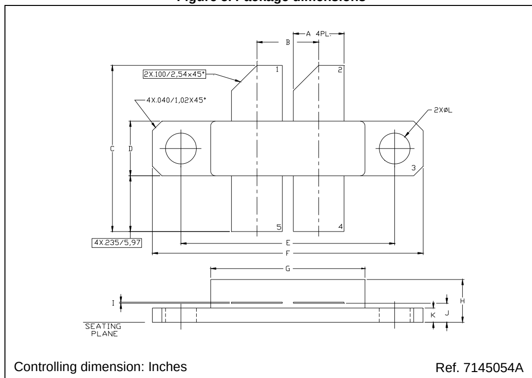
Figure 5. Package dimensions
