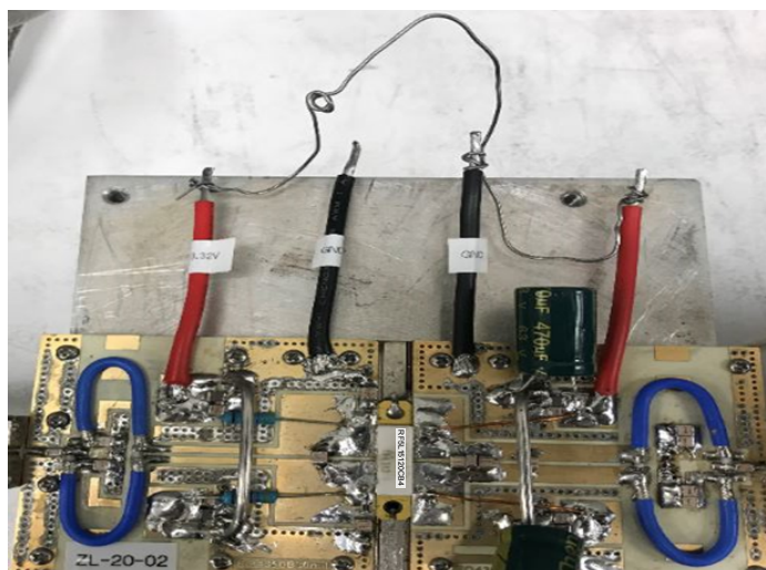
Figure 4. Test circuit photo (f = 1000 MHz)
