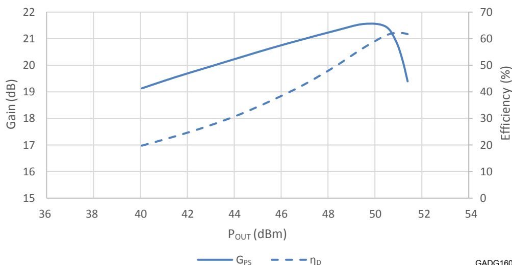
Figure 1. Power gain and drain efficiency versus output power (f = 1000 MHz, pulsed CW)
