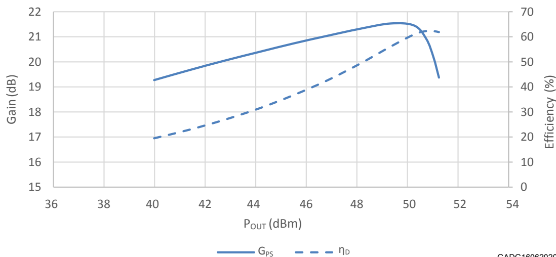
Figure 2. Power gain and drain efficiency versus output power (f = 1000 MHz, CW)
