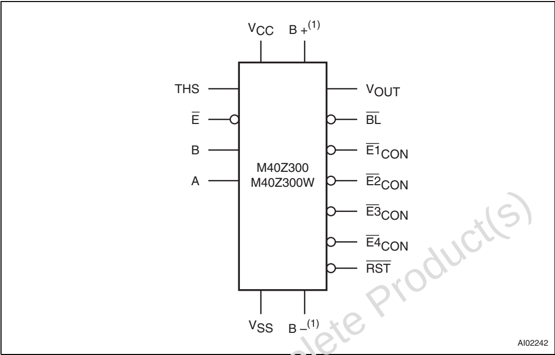
Figure 1. Logic diagram
