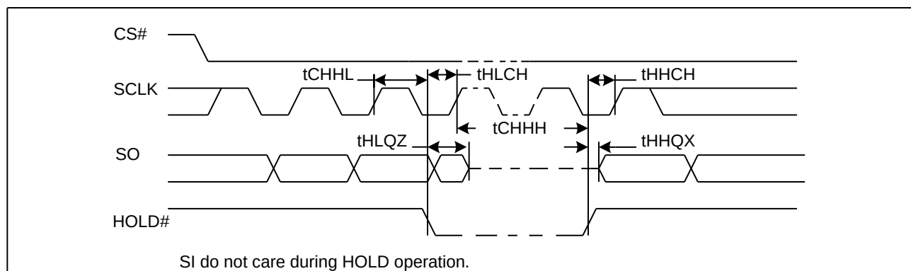
Figure 86. HOLD# Timing
