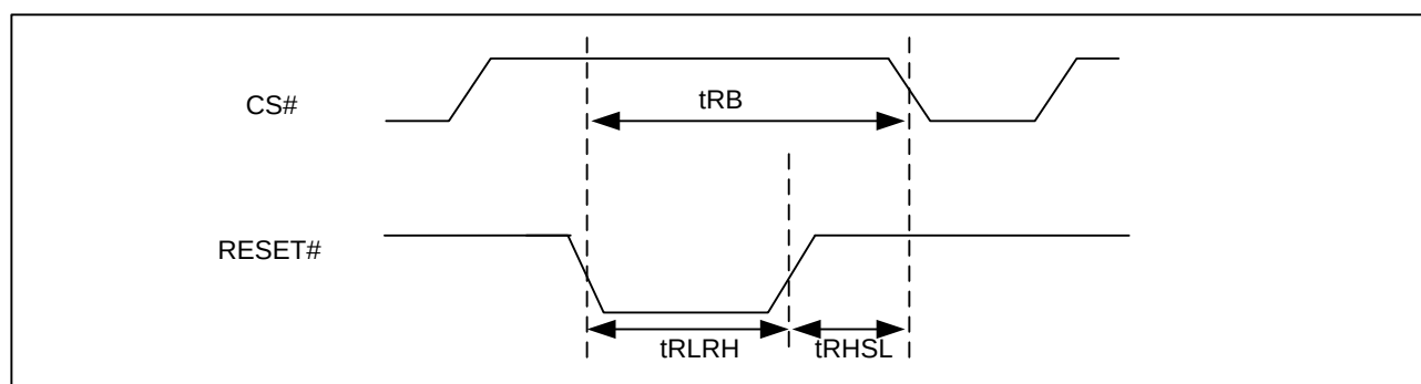
Figure 88 RESET# Timing
