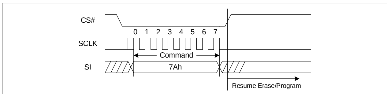
Figure 66. Program/Erase Resume Sequence Diagram (SPI)
