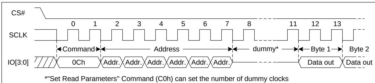
Figure 36. Burst Read with Wrap command Sequence Diagram
