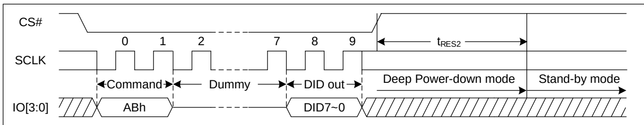
Figure 73. Release Power-Down/Read Device ID Sequence Diagram (QPI)
