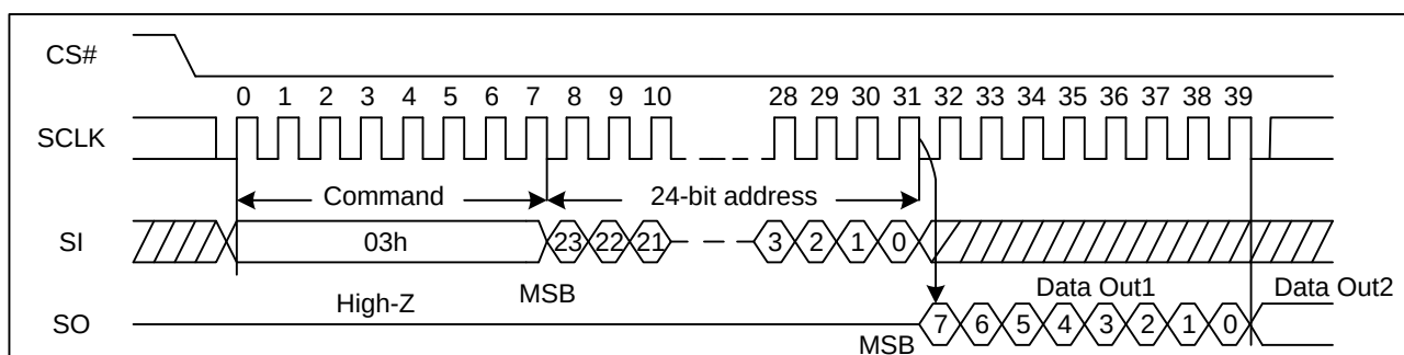
Figure 23. Read Data Bytes Sequence Diagram
