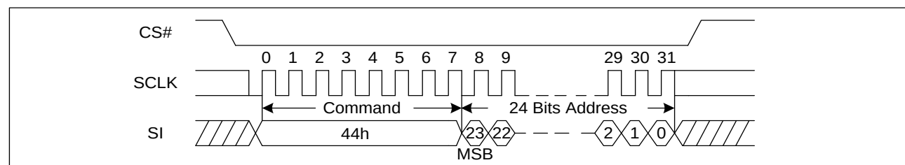
Figure 59. Erase Security Registers command Sequence Diagram
