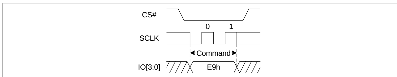
Figure 53 Disable 4-Byte Mode Sequence Diagram (QPI)
