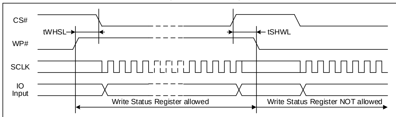
Figure 87. WP# Timing
