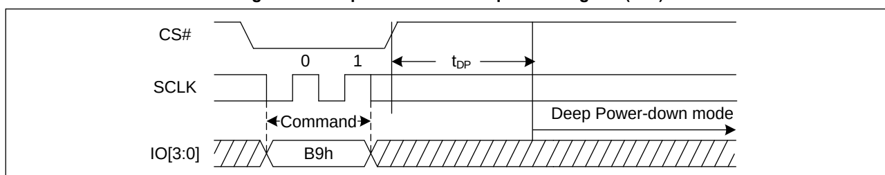
Figure 68. Deep Power-Down Sequence Diagram (QPI)
