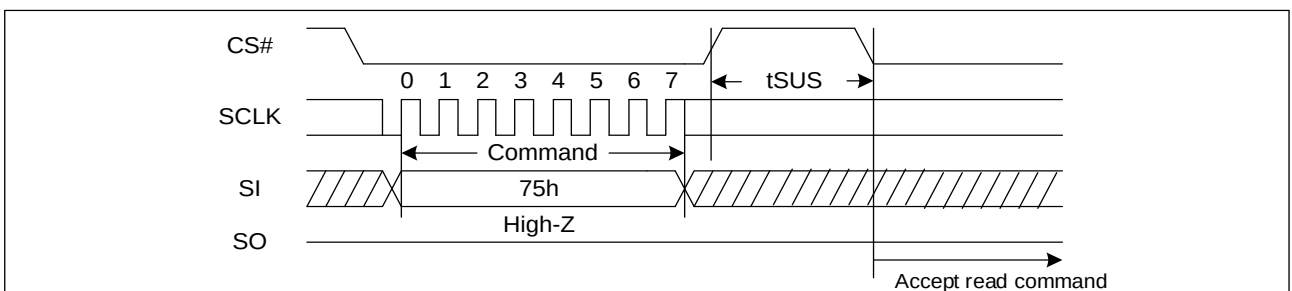
Figure 63. Program/Erase Suspend Sequence Diagram (SPI)
