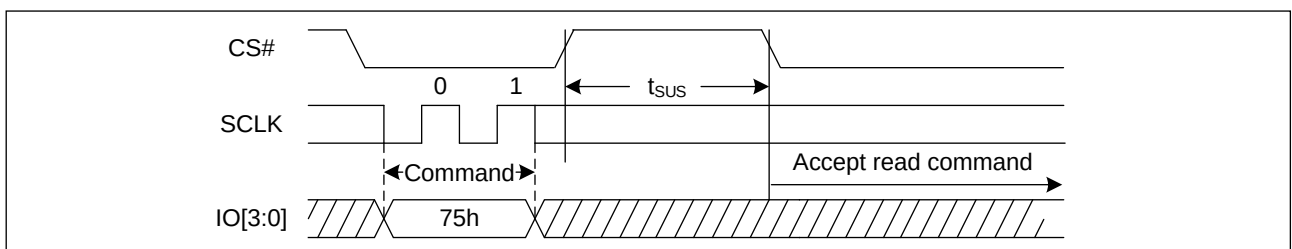
Figure 64. Program/Erase Suspend Sequence Diagram (QPI)
