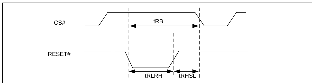
Figure 87 RESET# Timing
