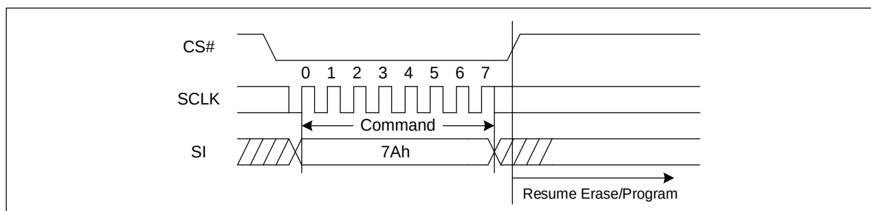
Figure 65. Program/Erase Resume Sequence Diagram (SPI)
