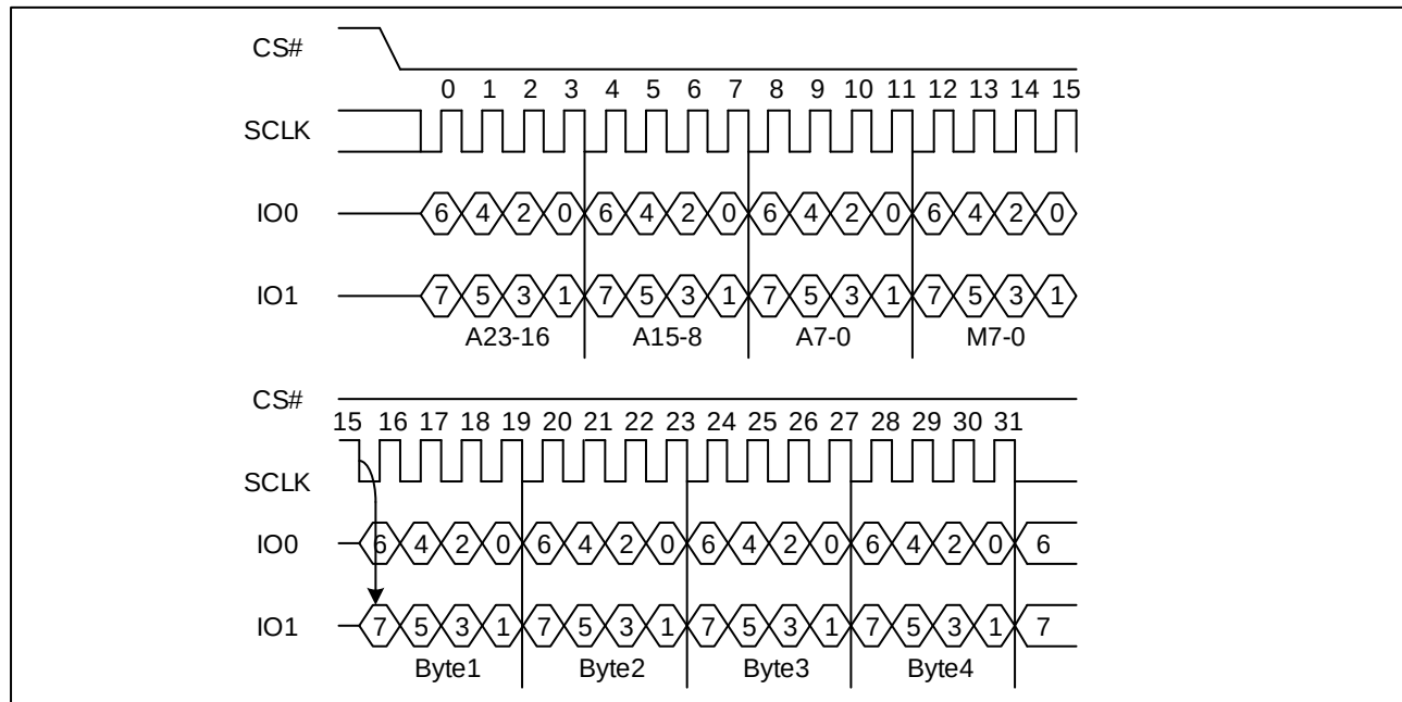
Figure 28. Dual I/O Fast Read Sequence Diagram ((M5-4) = (1, 0))
