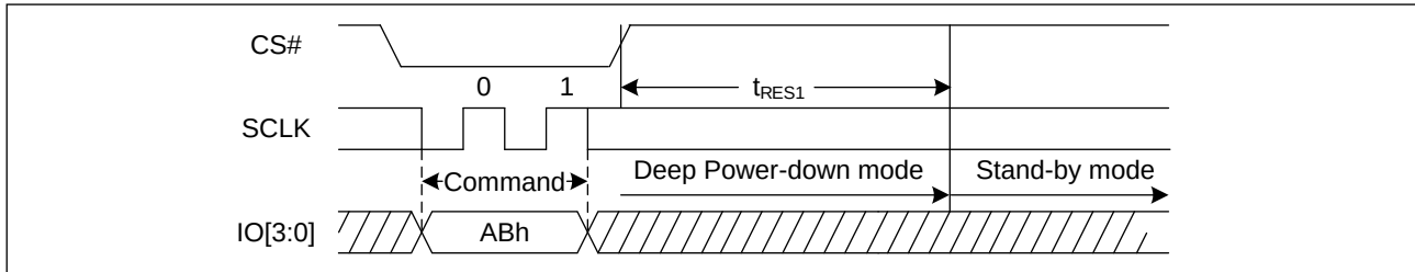
Figure 70. Release Power-Down Sequence Diagram (QPI)
