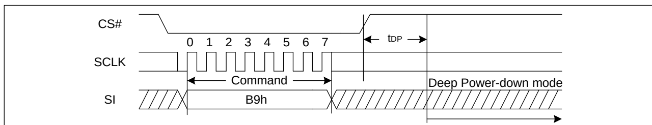
Figure 67. Deep Power-Down Sequence Diagram (SPI)
