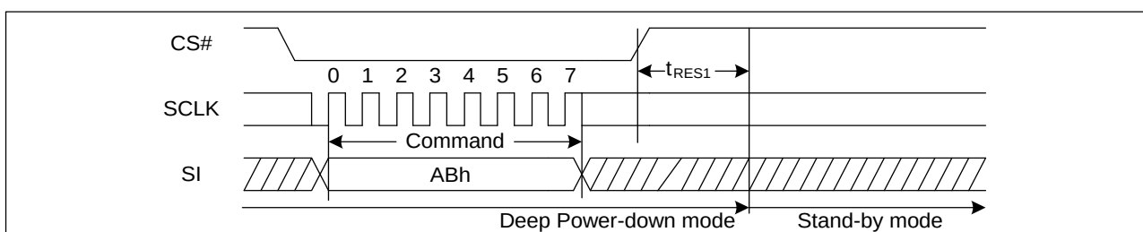
Figure 69. Release Power-Down Sequence Diagram (SPI)
