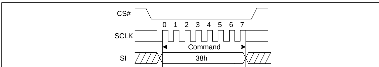
Figure 73. Enable QPI mode command Sequence Diagram
