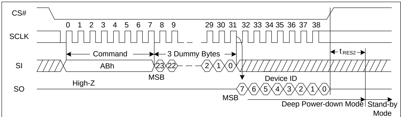
Figure 71. Release Power-Down/Read Device ID Sequence Diagram (SPI)
