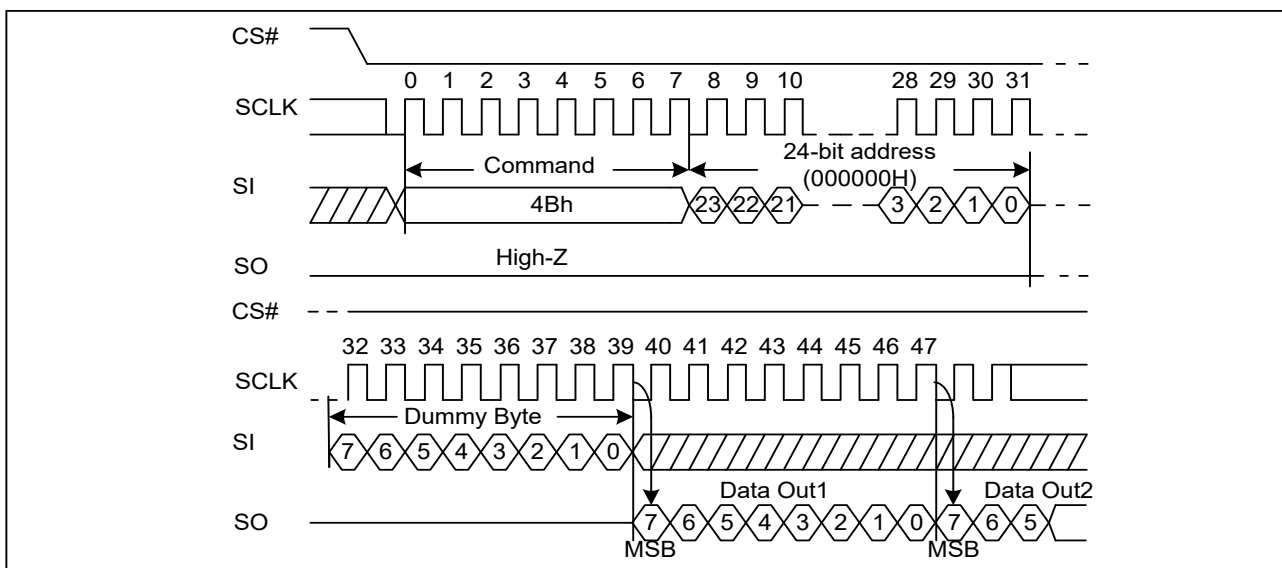
Figure 29. Read Unique ID Sequence Diagram
