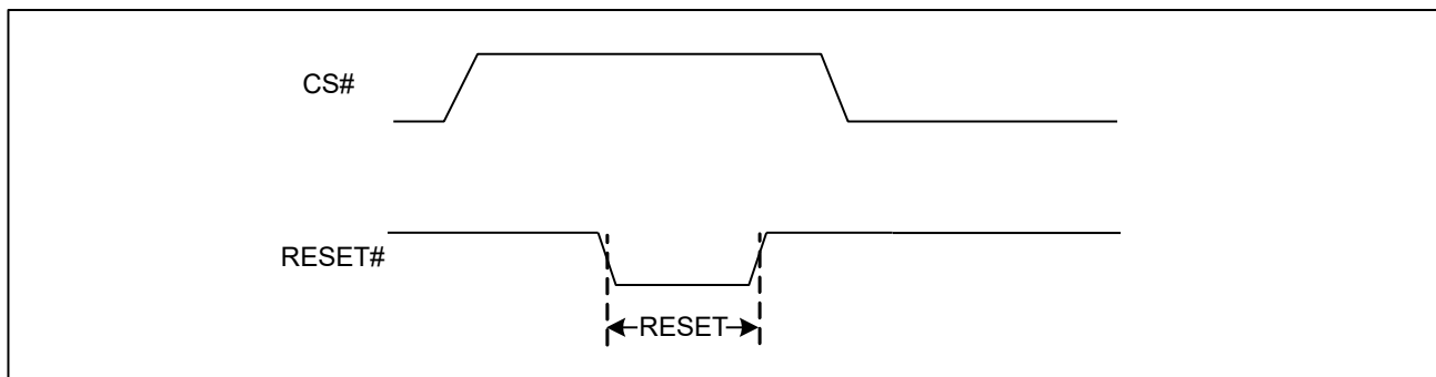
Figure 4 RESET Condition
