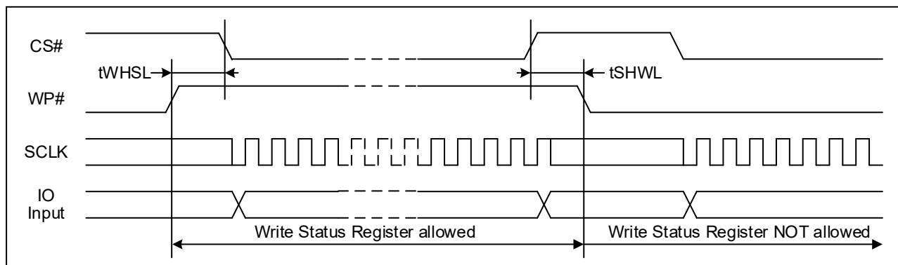
Figure 48. WP# Timing
