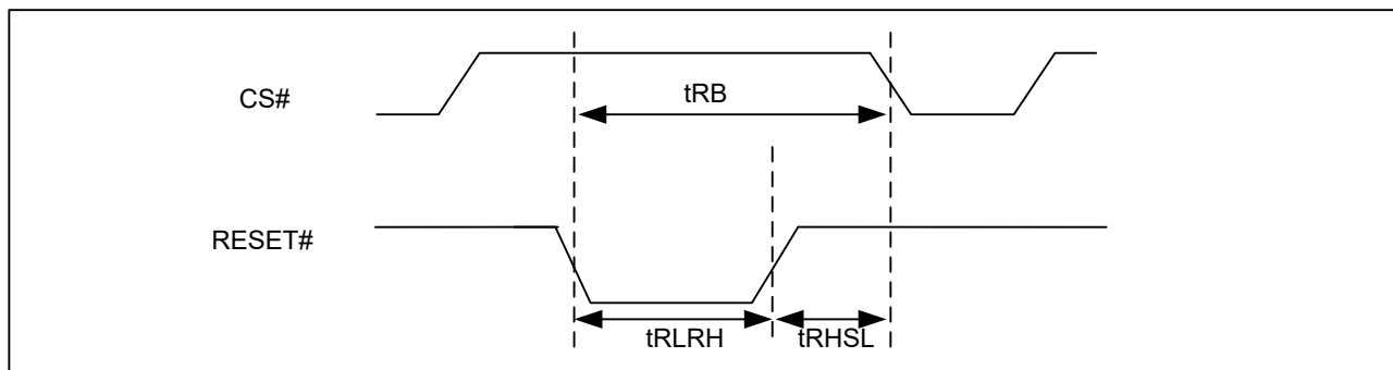
Figure 49 RESET Timing
