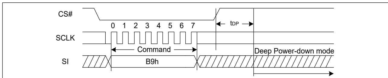
Figure 36. Deep Power-Down Sequence Diagram
