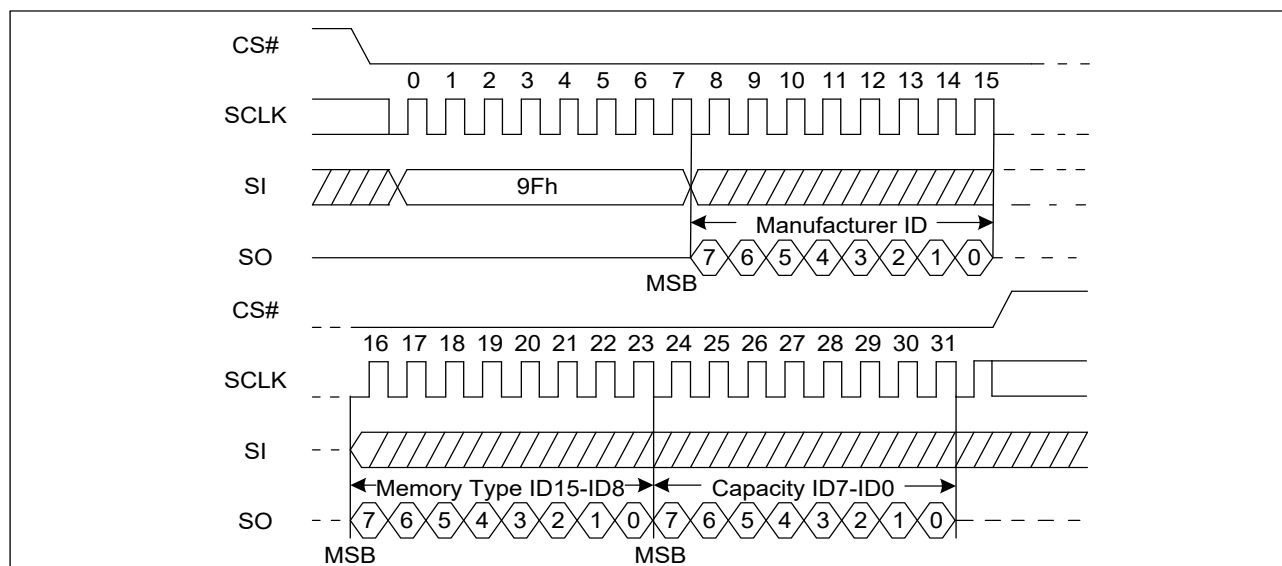
Figure 28. Read Identification ID Sequence Diagram
