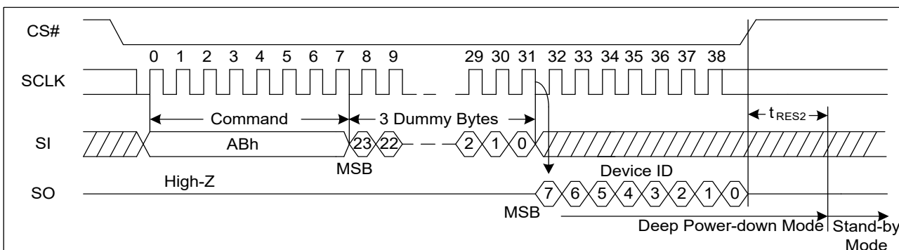
Figure 38. Release Power-Down/Read Device ID Sequence Diagram
