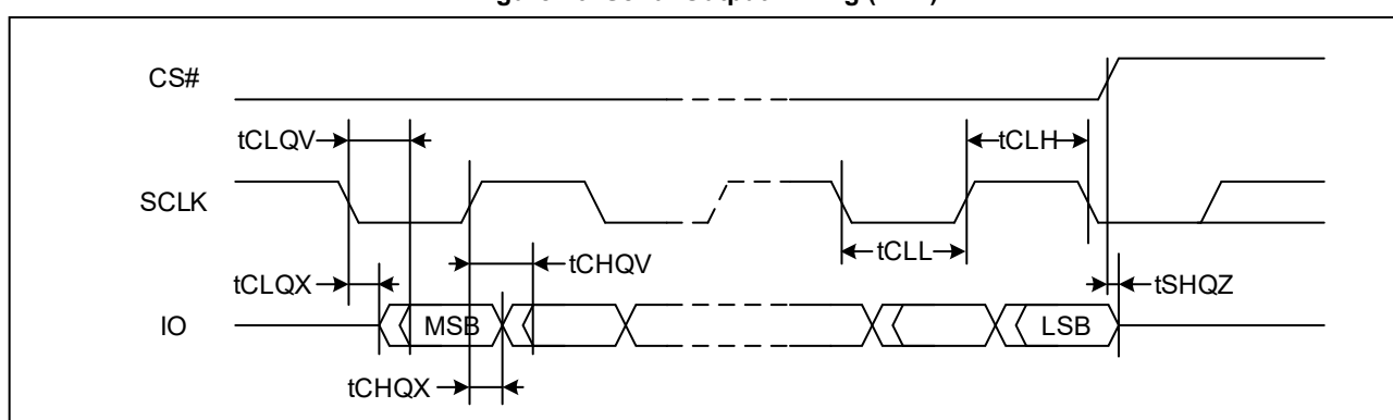
Figure 46. Serial Output Timing (DTR)
