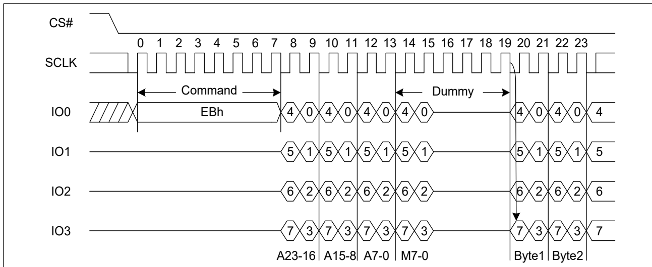
Figure 16. Quad I/O Fast Read Sequence Diagram ((M5-4) \neq (1, 0))
