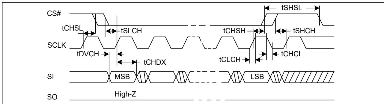
Figure 43. Input Timing
