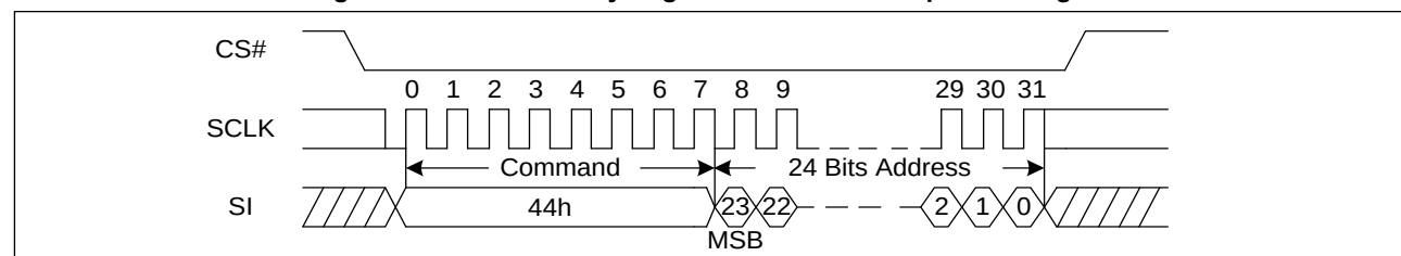
Figure 29. Erase Security Registers command Sequence Diagram
