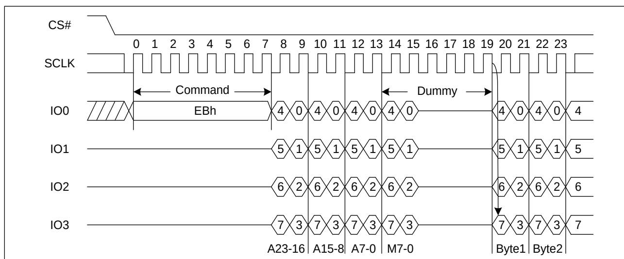
Figure 17. Quad I/O Fast Read Sequence Diagram ((M5-4) ≠ (1, 0))
