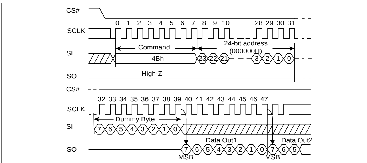
Figure 28. Read Unique ID Sequence Diagram
