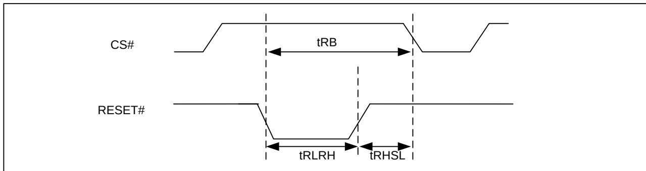
Figure 45. RESET# Timing
