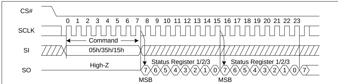
Figure 8. Read Status Register Sequence Diagram
