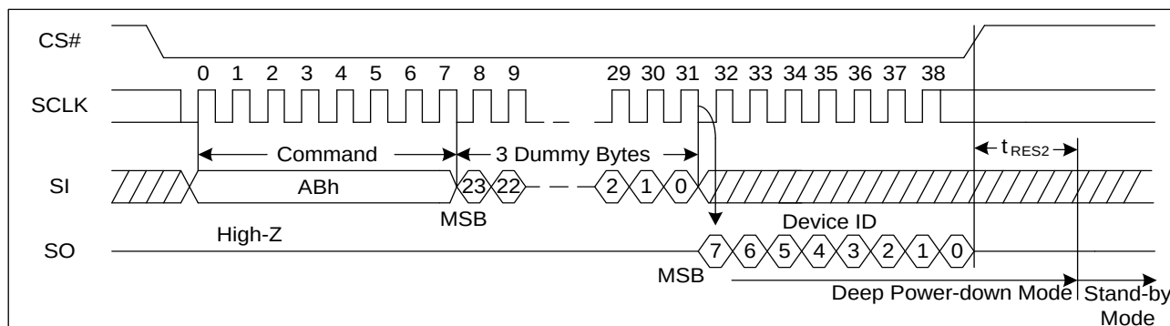
Figure 37. Release Power-Down/Read Device ID Sequence Diagram
