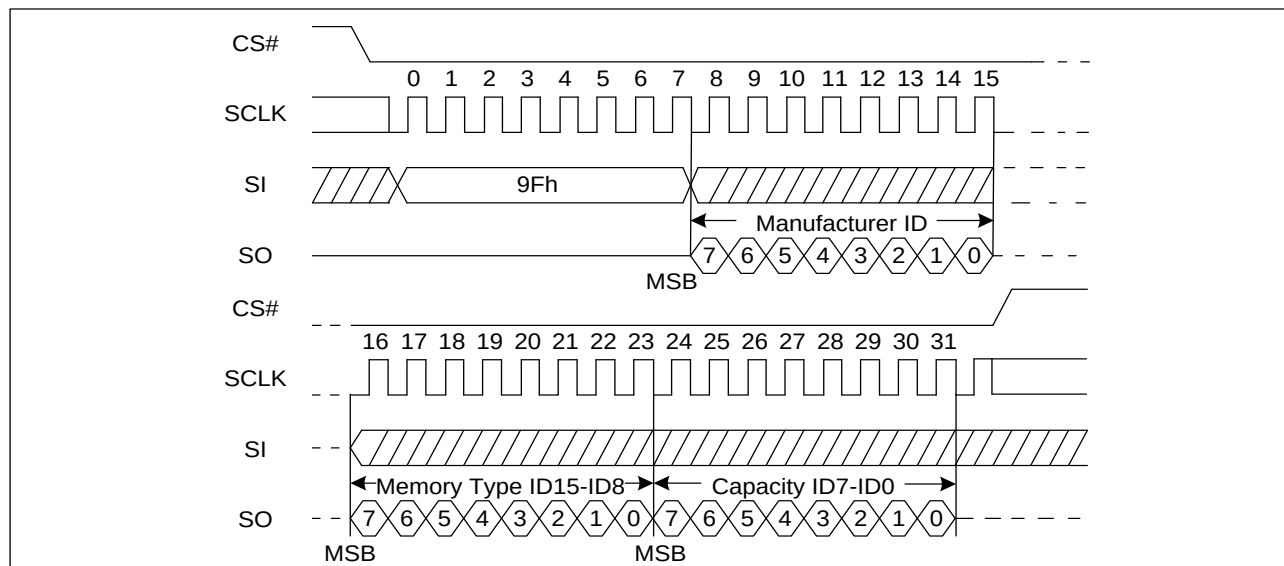
Figure 27. Read Identification ID Sequence Diagram
