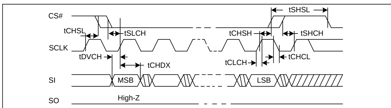
Figure 42. Input Timing
