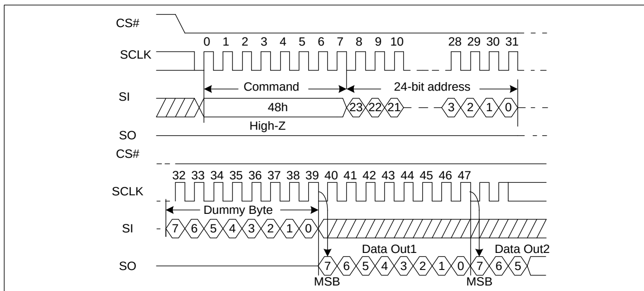
Figure 31. Read Security Registers command Sequence Diagram
