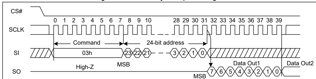
Figure 22. Read Data Bytes Sequence Diagram
