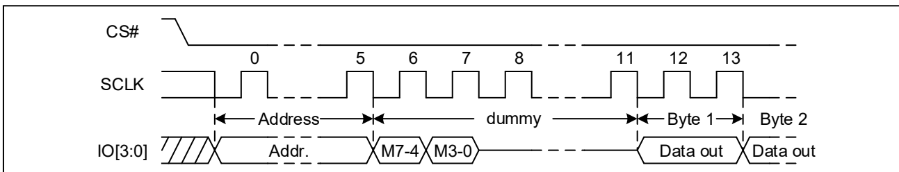
Figure 33. Quad I/O Fast Read Sequence Diagram ((M5-4) = (1, 0))
