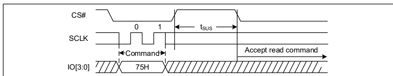
Figure 53. Program/Erase Suspend Sequence Diagram (QPI)
