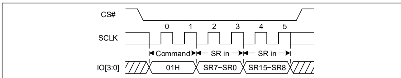
Figure 12. Write Status Register Sequence Diagram (QPI)
