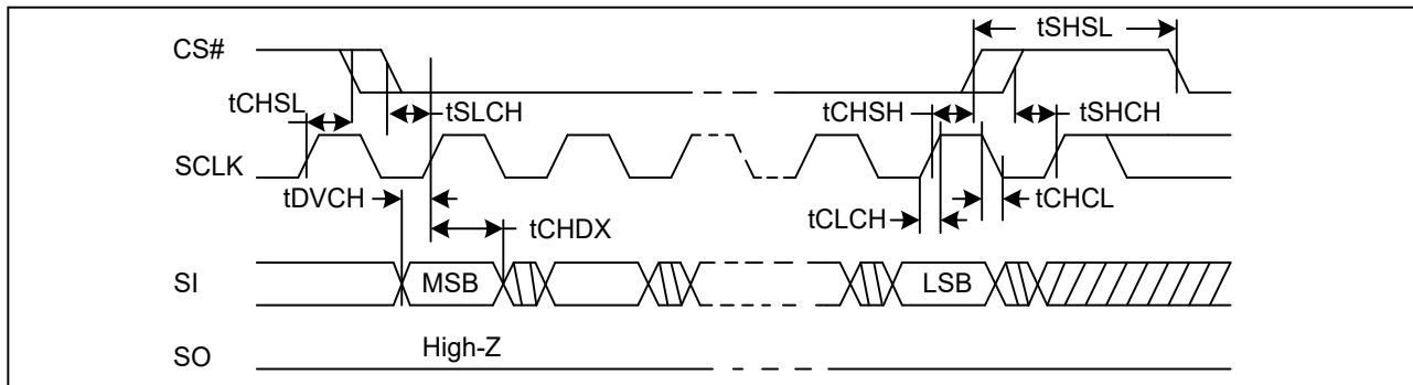
Figure 69. Input Timing
