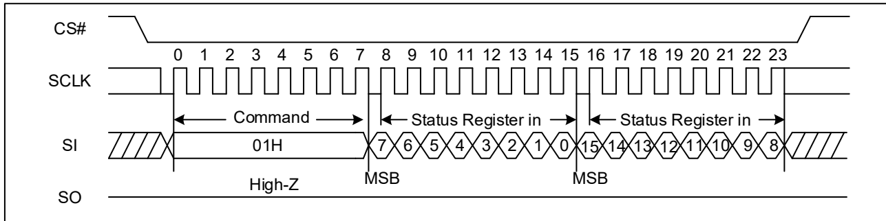
Figure 11. Write Status Register Sequence Diagram (SPI)
