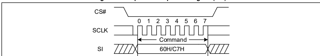
Figure 38. Chip Erase Sequence Diagram (SPI)
