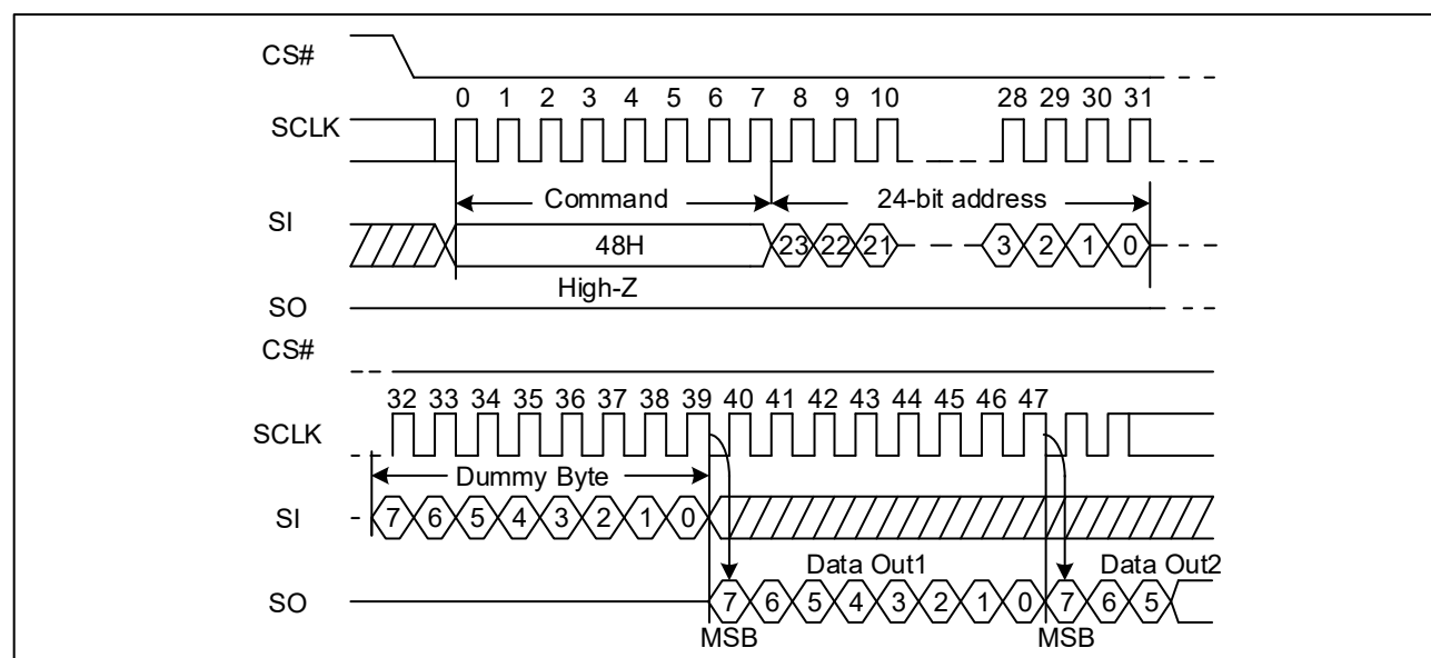
Figure 48. Read Security Registers command Sequence Diagram
