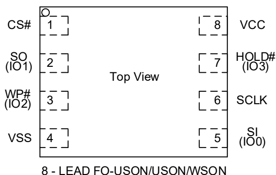
Figure 2 Connection Diagram for FO-USON8/USON8/WSON8 package
