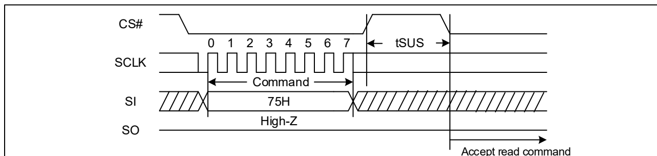
Figure 52. Program/Erase Suspend Sequence Diagram (SPI)
