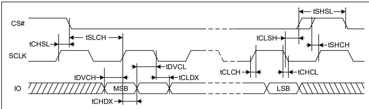
Figure 71. Serial Input Timing (DTR)
