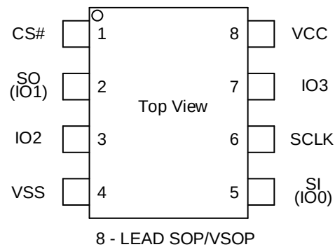
Figure 2 Connection Diagram for SOP8/VSOP8 package
