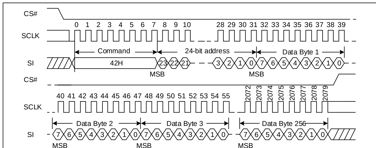
Figure 42. Program Security Registers command Sequence Diagram
