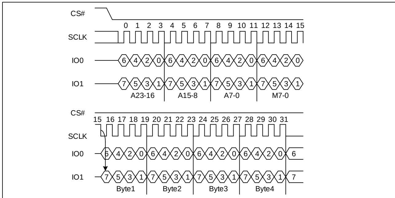
Figure 19. Dual I/O Fast Read Sequence Diagram (M5-4 = (1, 0))
