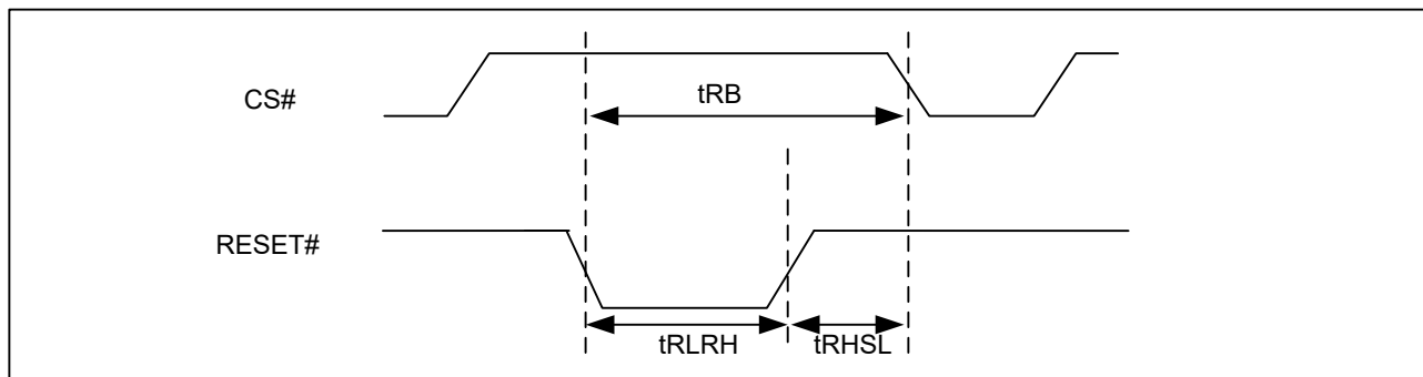
Figure 85. RESET# Timing
