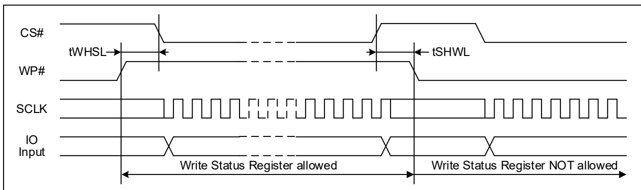
Figure 84. WP# Timing
