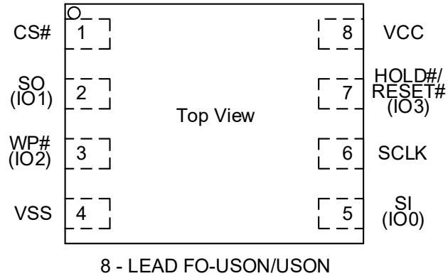
Figure 2 Connection Diagram for FO-USON8/USON8 package
