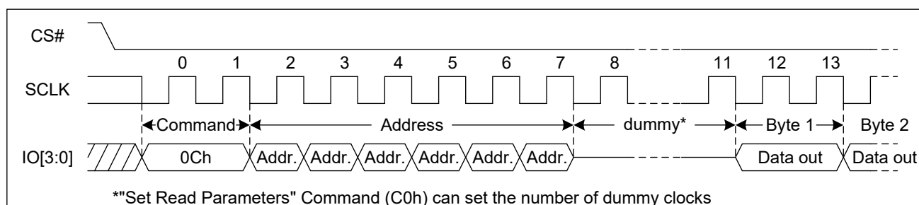
Figure 34. Burst Read with Wrap Sequence Diagram
