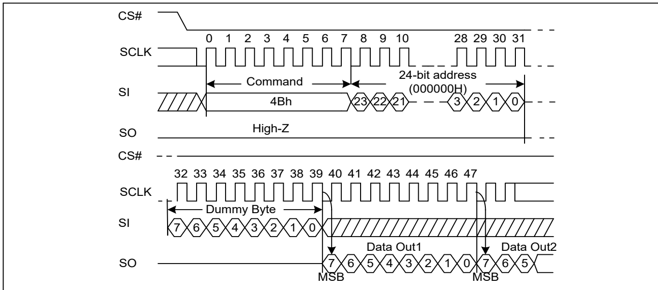
Figure 53. Read Unique ID Sequence Diagram
