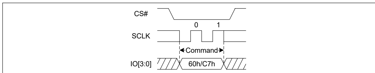
Figure 48. Chip Erase Sequence Diagram (QPI)
