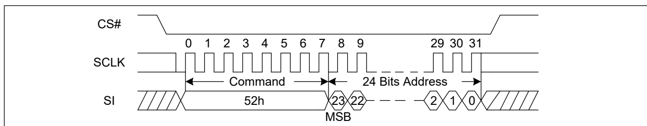
Figure 43. 32KB Block Erase Sequence Diagram (SPI)
