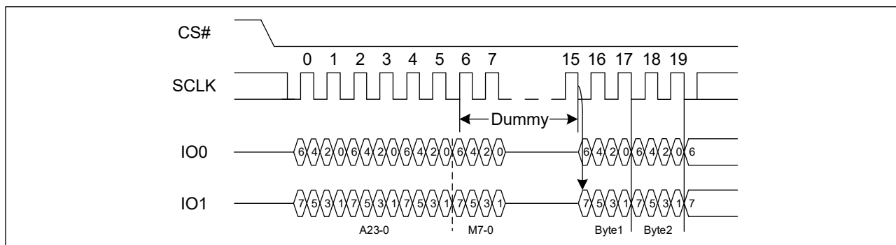
Figure 30. DTR Dual I/O Fast Read Sequence Diagram (M5-4 = (1, 0))
