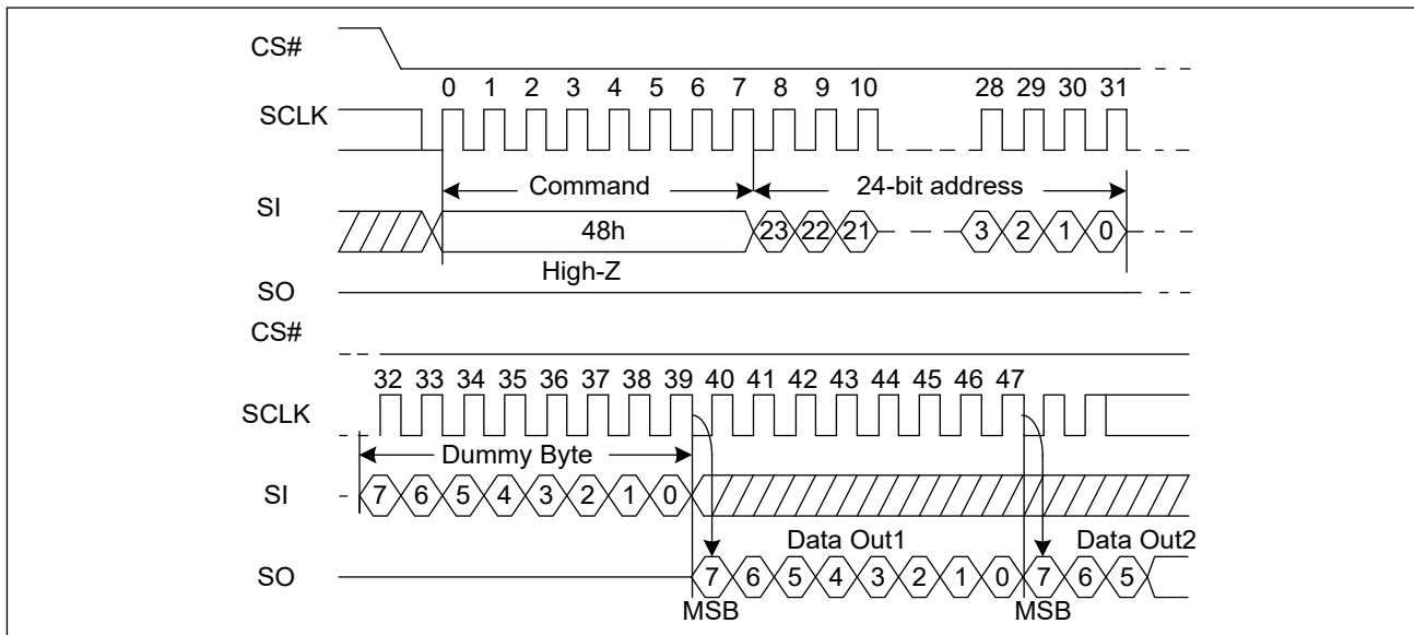
Figure 56. Read Security Registers command Sequence Diagram
