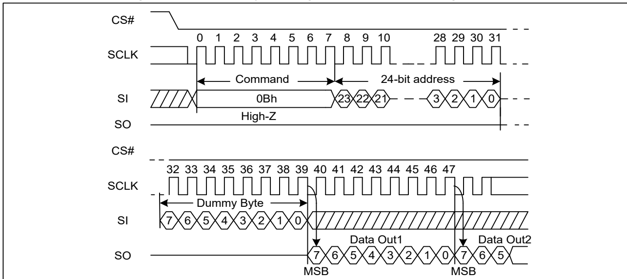
Figure 20. Read Data Bytes at Higher Speed Sequence Diagram (SPI)
