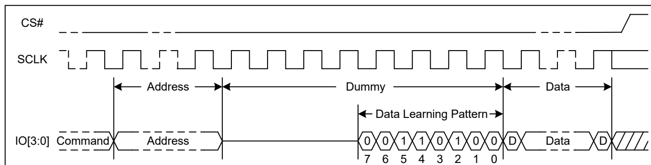
Figure 4. Data Learning Pattern Sequence Diagram (DTR, Dummy Clock ≥ 8)
