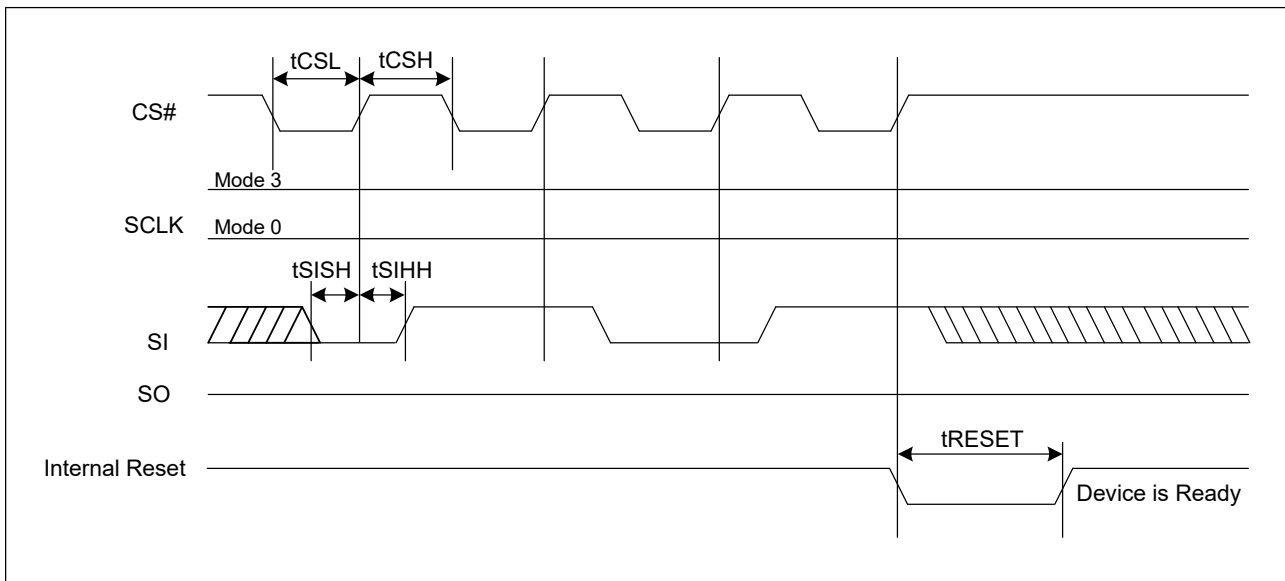
Figure 3. JEDEC RESET Signaling Protocol
