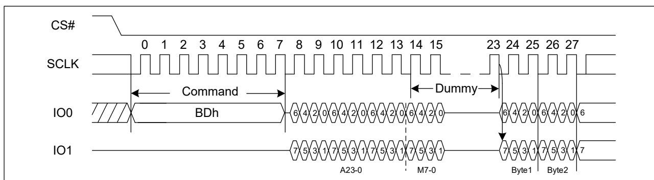
Figure 29. DTR Dual I/O Fast Read Sequence Diagram (M5-4 ≠ (1, 0))
