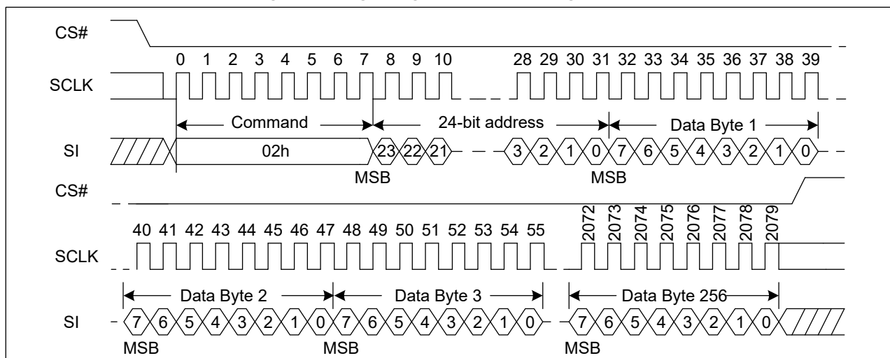
Figure 38. Page Program Sequence Diagram (SPI)
