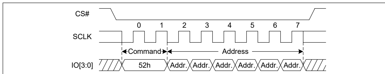
Figure 44. 32KB Block Erase Sequence Diagram (QPI)
