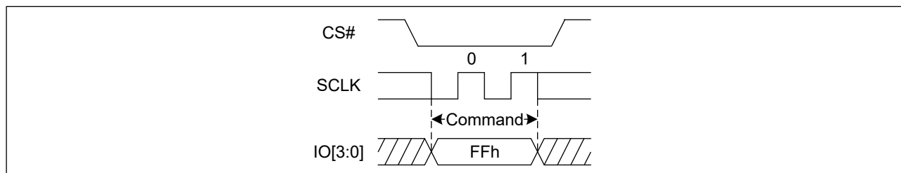
Figure 70. Disable QPI mode command Sequence Diagram
