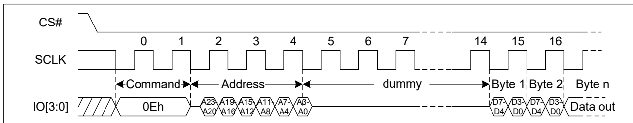
Figure 35. DTR Burst Read with Wrap Sequence Diagram
