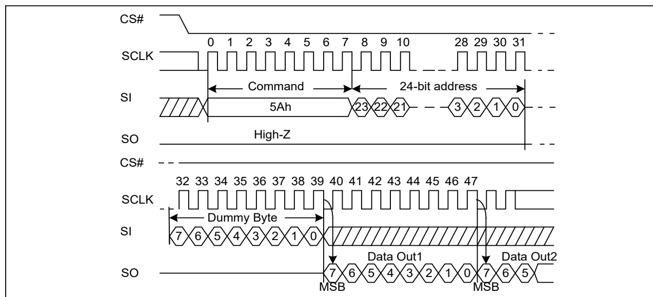
Figure 71. Read Serial Flash Discoverable Parameter command Sequence Diagram
