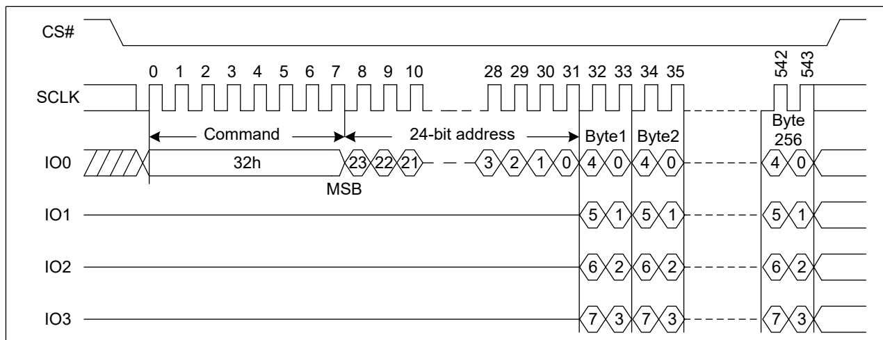
Figure 40. Quad Page Program Sequence Diagram
