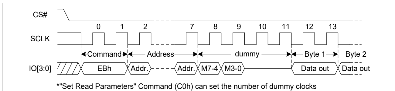
Figure 27. Quad I/O Fast Read Sequence Diagram ((M5-4) ≠ (1, 0), QPI)
