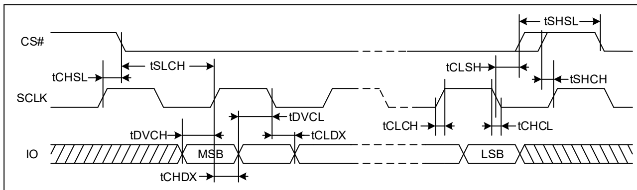
Figure 77. Serial Input Timing (DTR)
