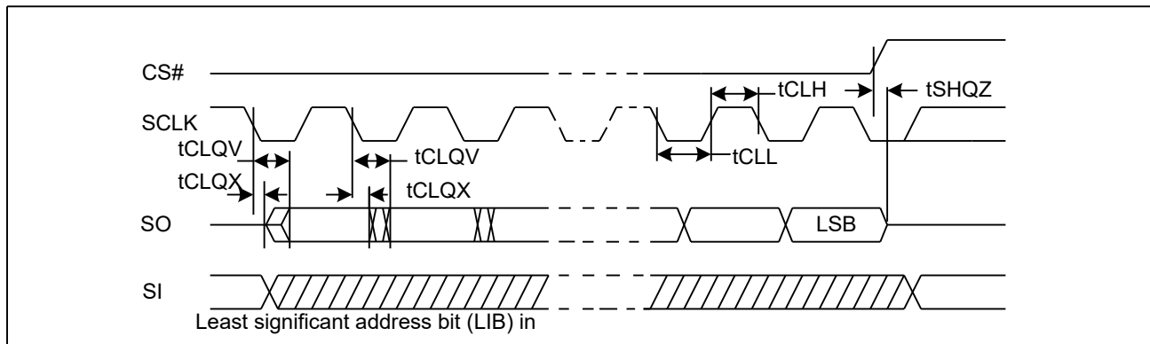
Figure 76. Serial Output Timing (STR)
