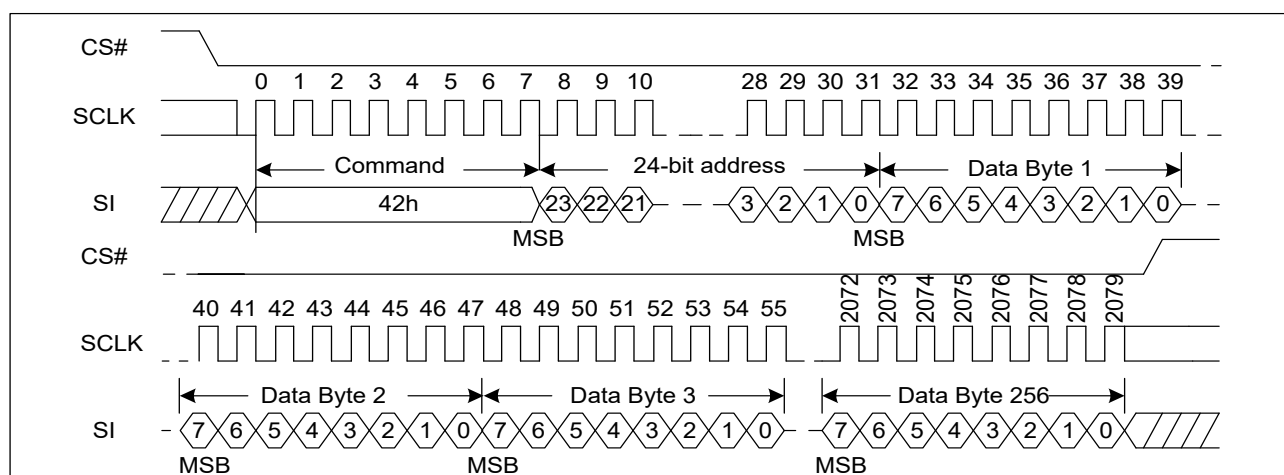
Figure 55. Program Security Registers command Sequence Diagram
