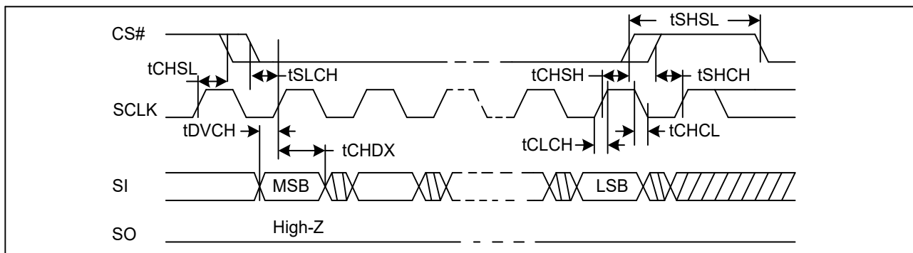
Figure 75. Serial Input Timing (STR)
