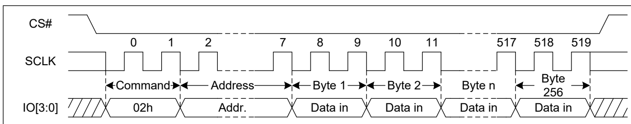
Figure 39. Page Program Sequence Diagram (QPI)
