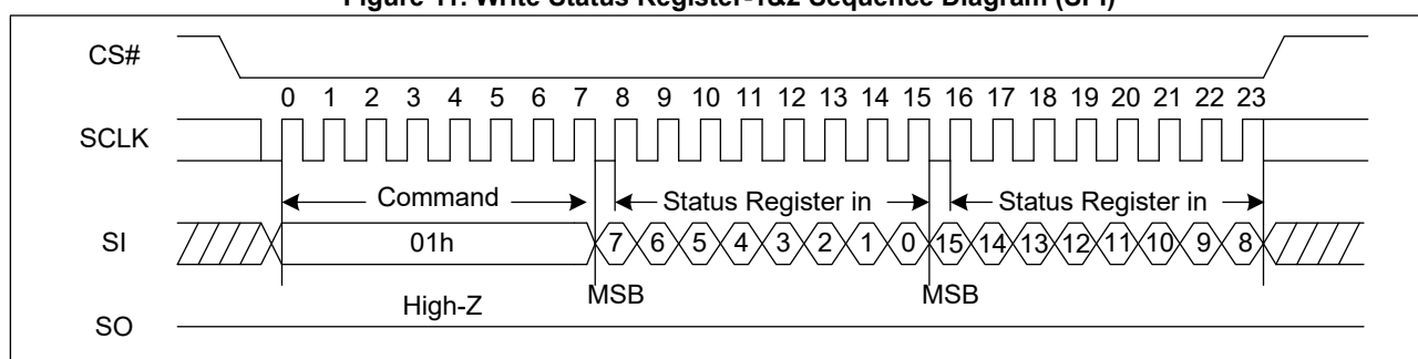
Figure 11. Write Status Register-1&2 Sequence Diagram (SPI)
