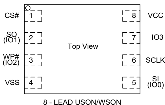
Figure 1 Connection Diagram for USON8/WSO8 package
