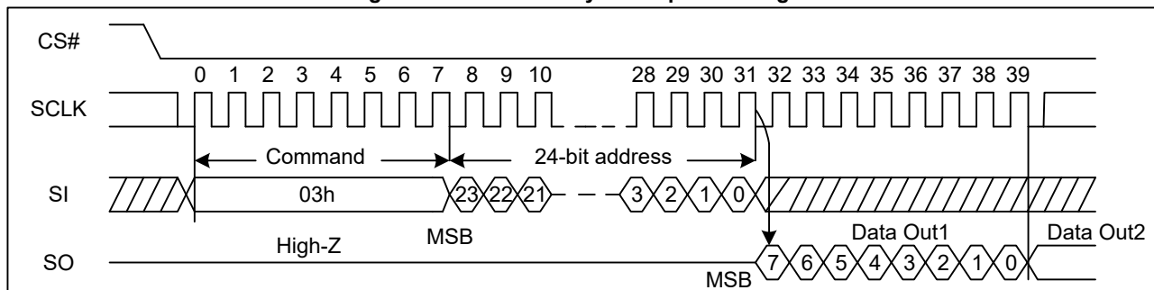
Figure 19. Read Data Bytes Sequence Diagram
