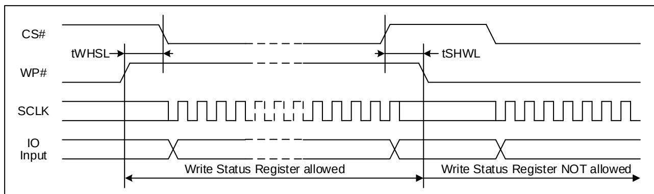
Figure 72. WP# Timing
