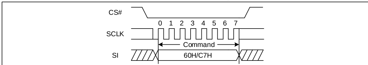
Figure 35. Chip Erase Sequence Diagram (SPI)
