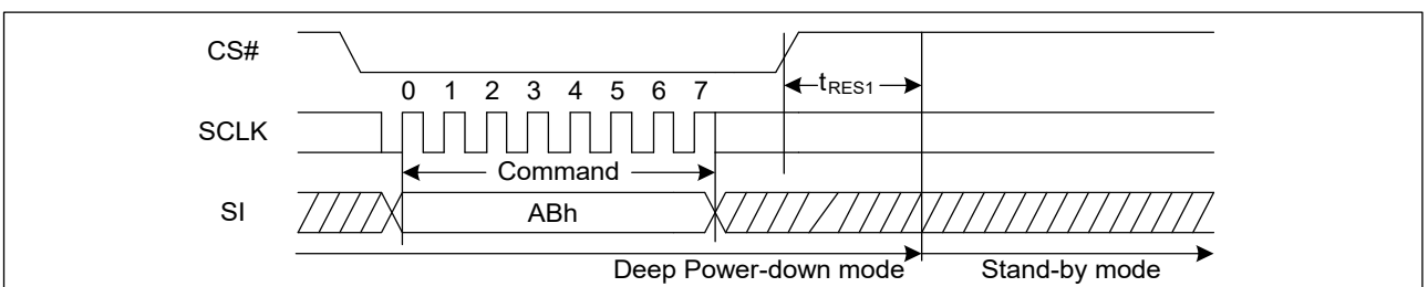
Figure 67. Release Power-Down Sequence Diagram (SPI)
