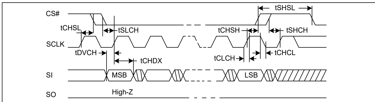
Figure 77. Serial Input Timing (STR)
