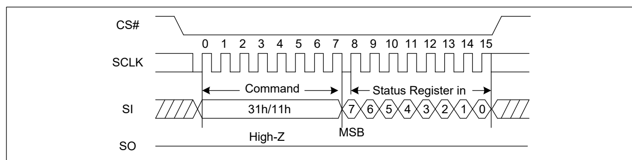
Figure 15. Write Status Register Sequence Diagram (SPI)
