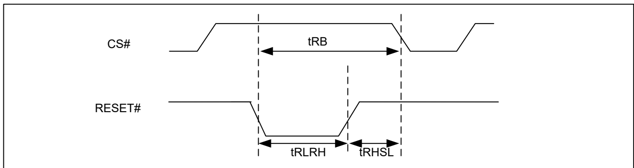
Figure 84. RESET# Timing
