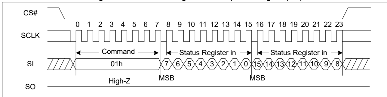
Figure 14. Write Status Register-1&2 Sequence Diagram (SPI)
