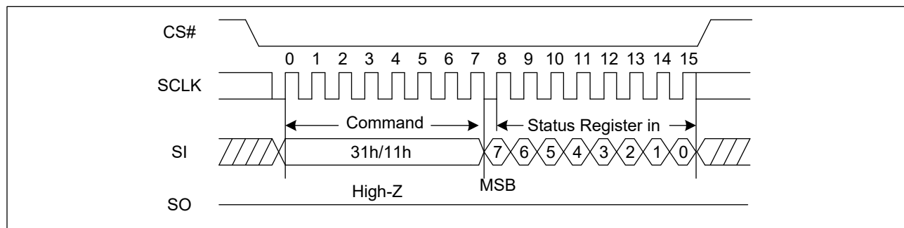
Figure 16. Write Status Register Sequence Diagram (SPI)
