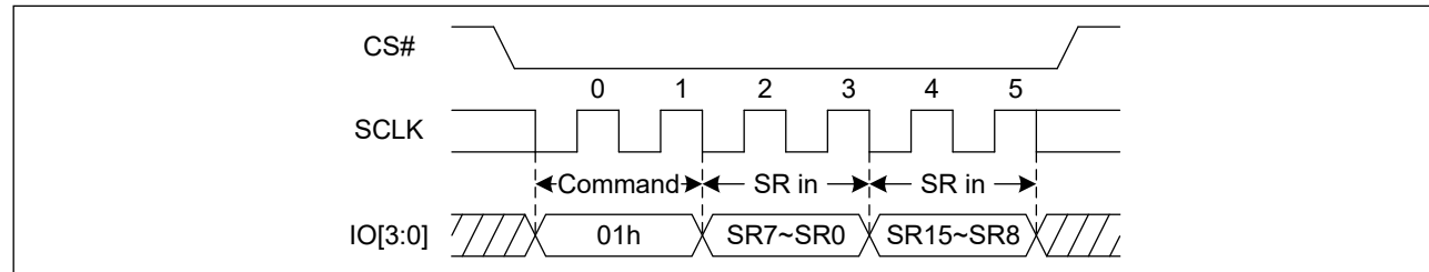
Figure 15. Write Status Register-1&2 Sequence Diagram (QPI)
