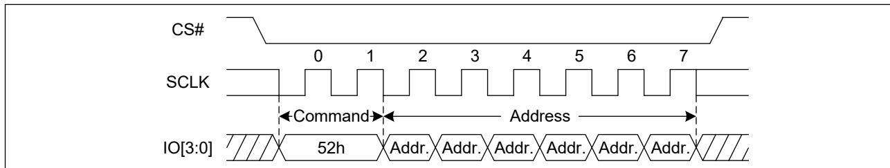
Figure 47. 32KB Block Erase Sequence Diagram (QPI)
