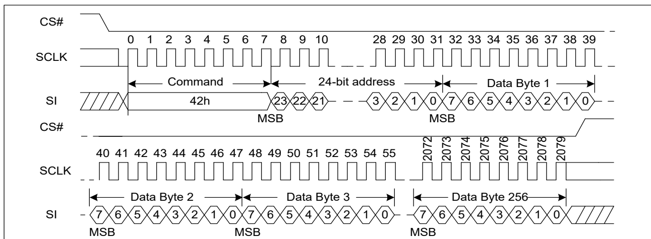
Figure 58. Program Security Registers command Sequence Diagram
