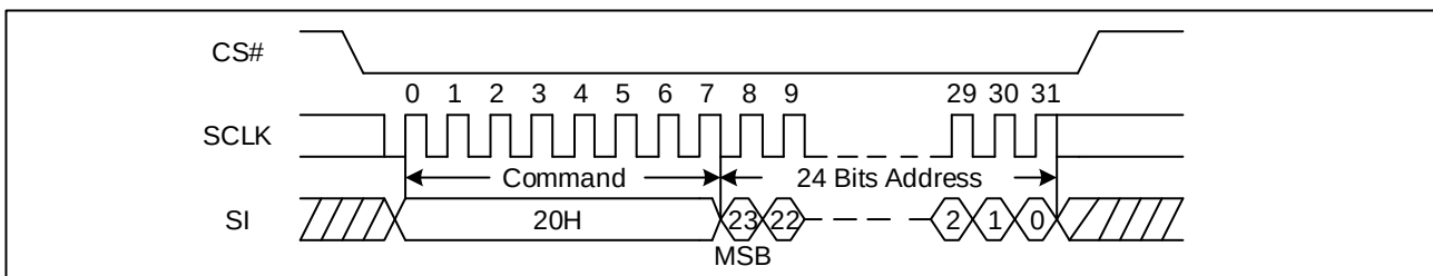
Figure 12. Sector Erase Sequence Diagram
