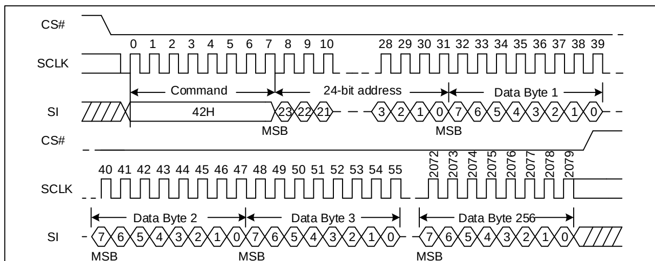
Figure 20. Program Security Registers command Sequence Diagram
