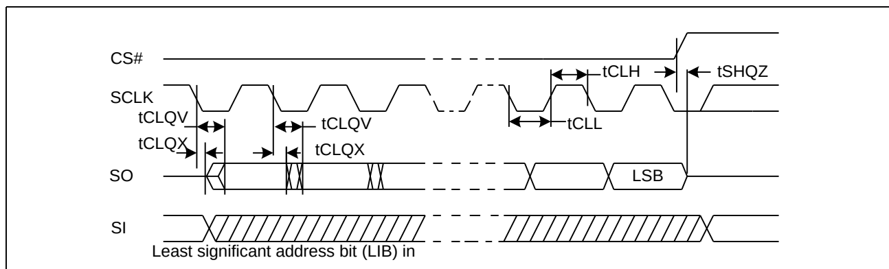
Figure 29. Output Timing
