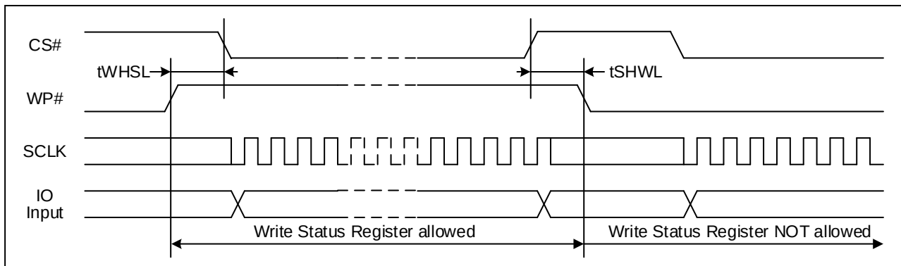
Figure 30. WP# Timing
