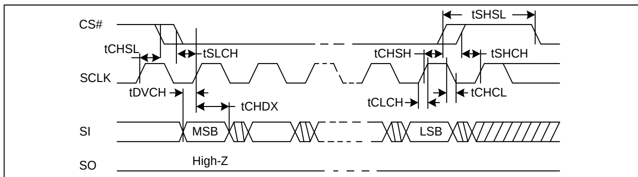
Figure 28. Input Timing
