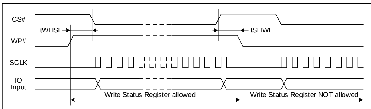
Figure 30. WP# Timing
