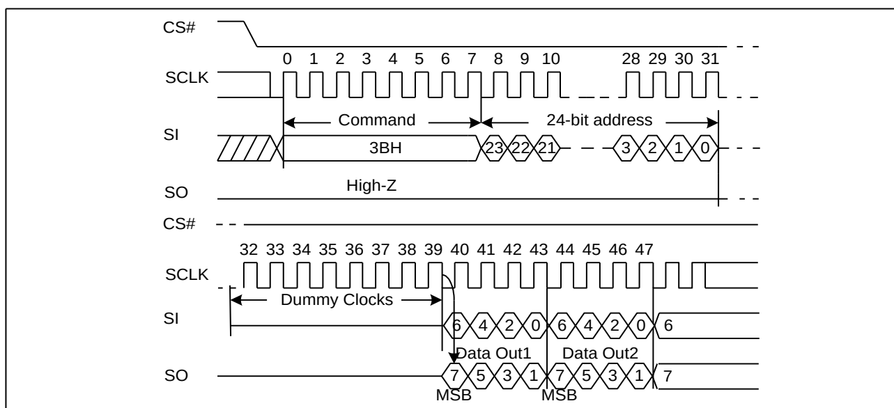
Figure 16. Dual Output Fast Read Sequence Diagram (ADS=0)
