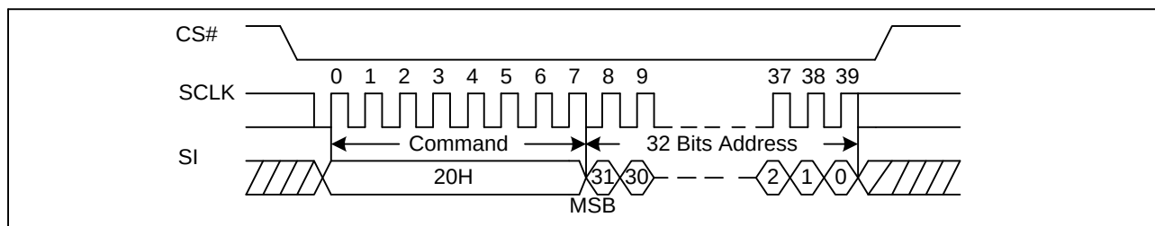
Figure 49. Sector Erase Sequence Diagram (ADS=1)
