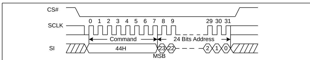
Figure 72. Erase Security Registers command Sequence Diagram (ADS=0)
