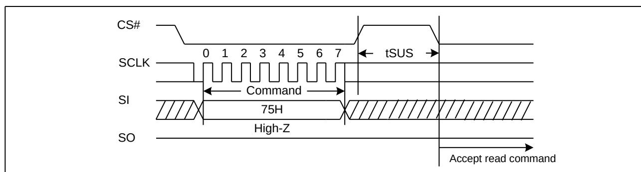
Figure 70. Program/Erase Suspend Sequence Diagram
