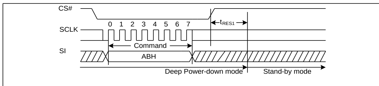
Figure 64. Release Power-Down Sequence Diagram
