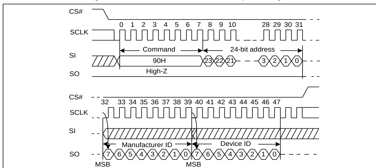
Figure 66. Read Manufacture ID/ Device ID Sequence Diagram
