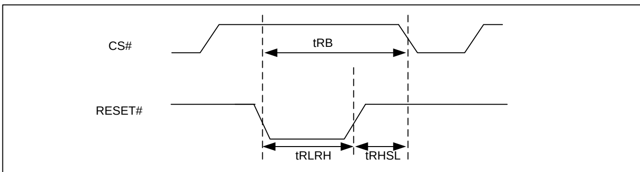
Figure 86 RESET Timing
