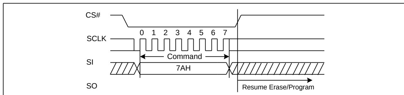
Figure 71. Program/Erase Resume Sequence Diagram
