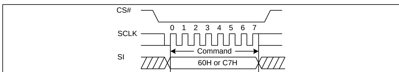
Figure 57. Chip Erase Sequence Diagram
