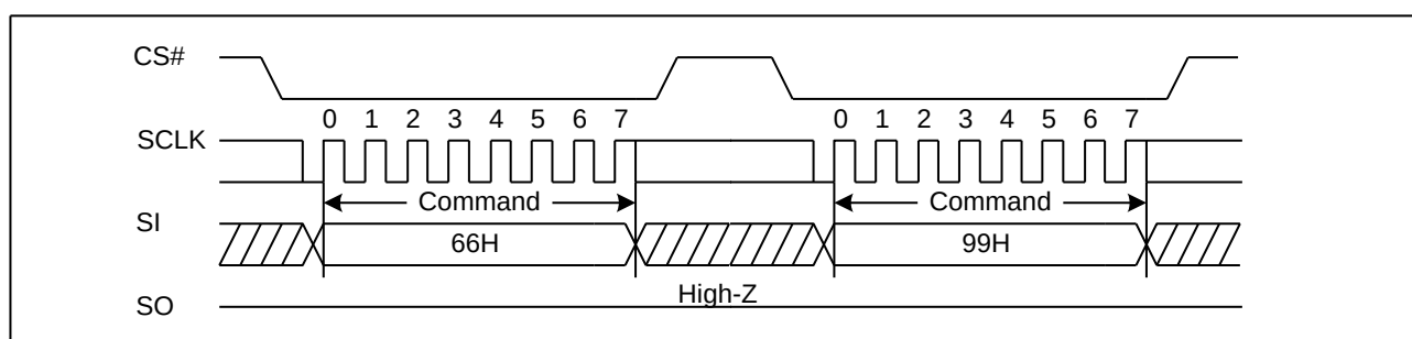
Figure 78. Enable Reset and Reset command Sequence Diagram
