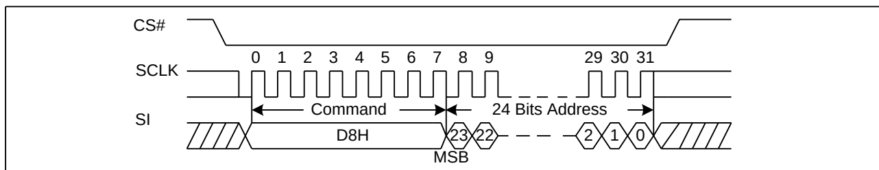
Figure 55. 64KB Block Erase Sequence Diagram (ADS=1)
