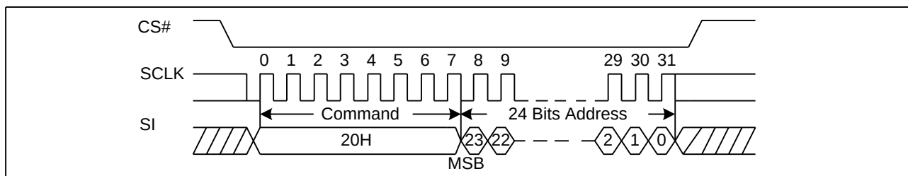
Figure 48. Sector Erase Sequence Diagram (ADS=0)
