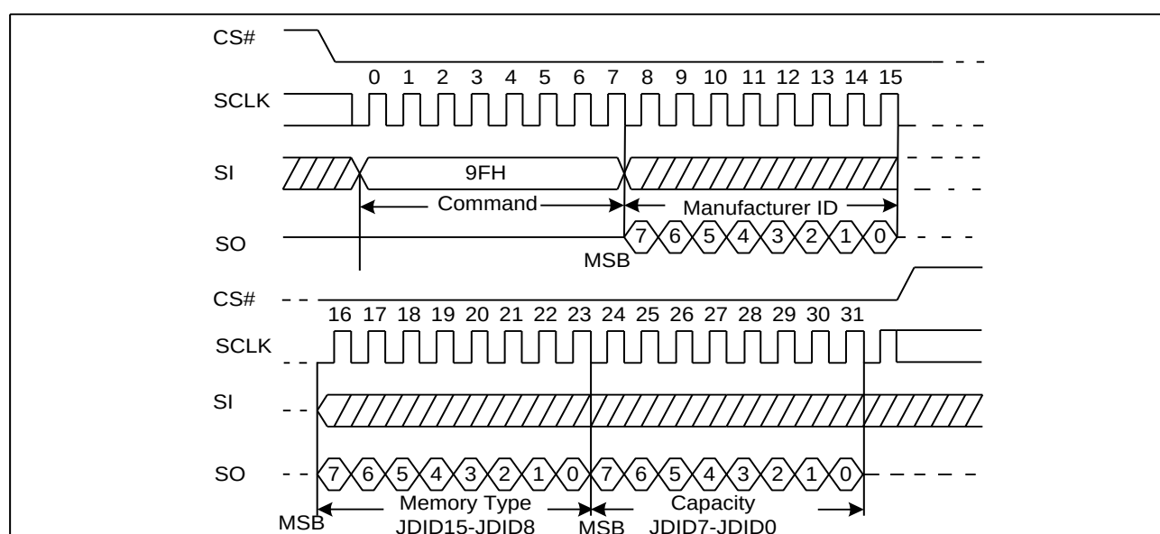
Figure 69. Read Identification ID Sequence Diagram
