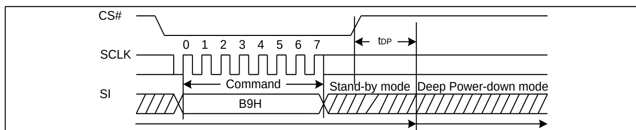
Figure 58. Deep Power-Down Sequence Diagram
