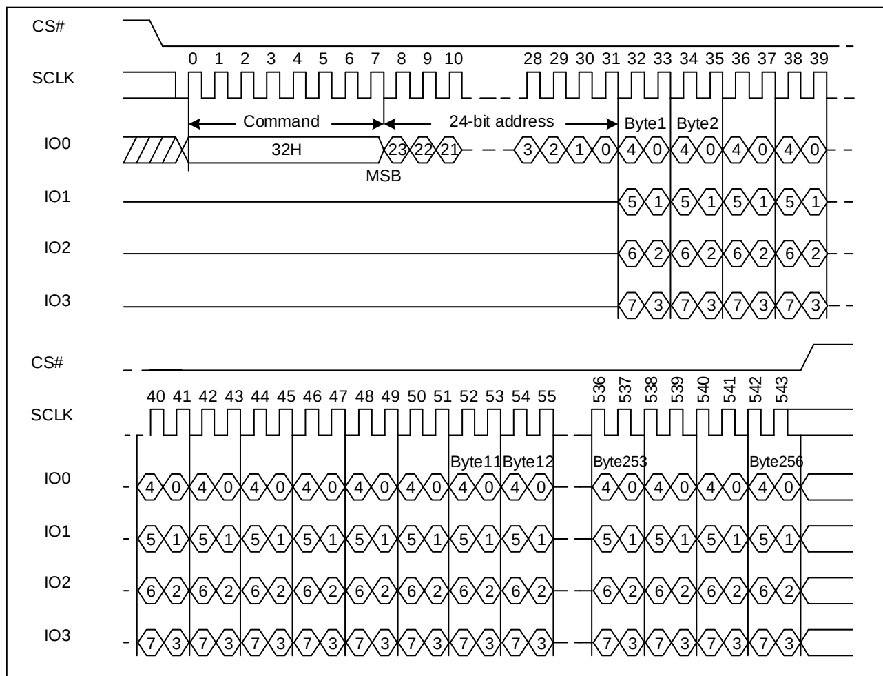
Figure 45. Quad Page Program Sequence Diagram (ADS=0)
