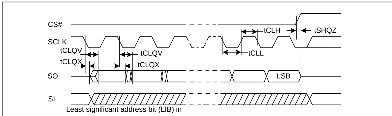
Figure 84. Output Timing
