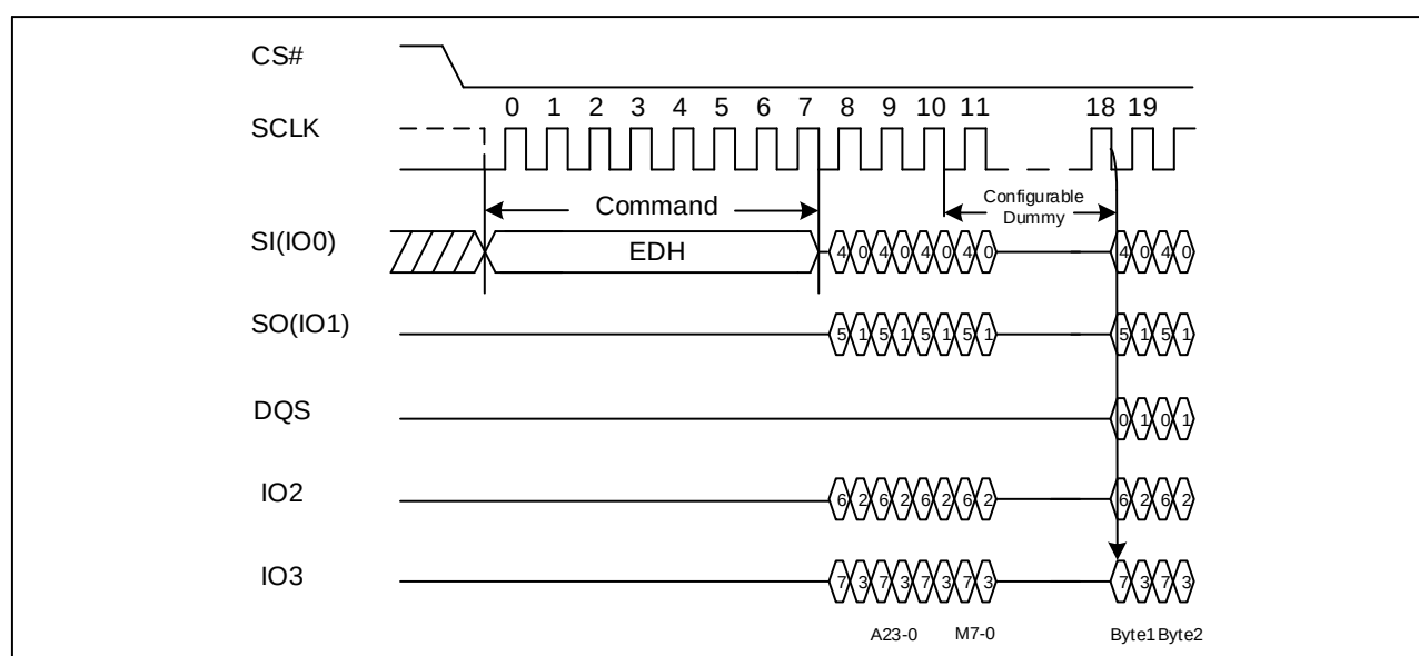
Figure 35. DTR Quad I/O Fast Read Sequence Diagram (ADS=0)
