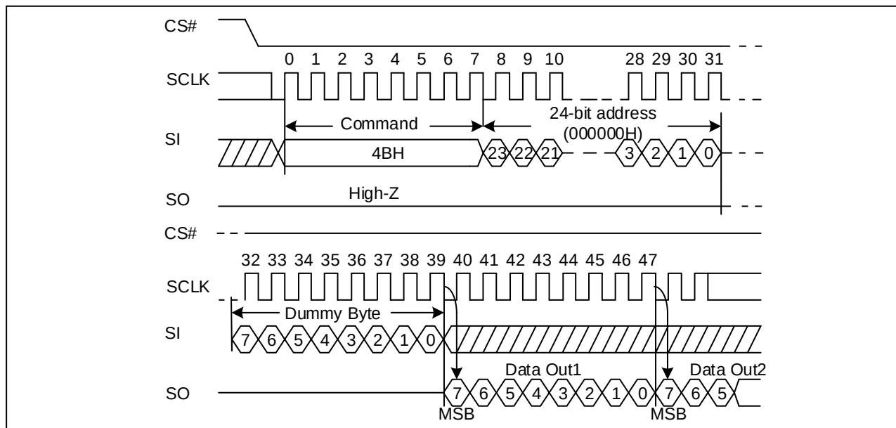
Figure32. Read Unique ID Sequence Diagram
