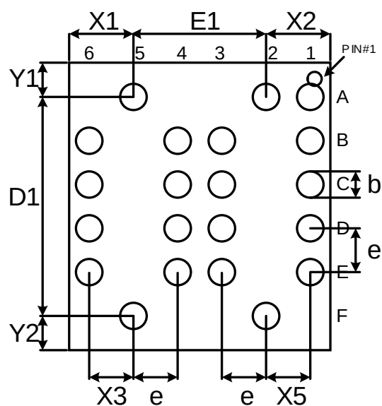
BOTTOM VIEW
