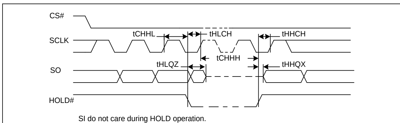
Figure47. Hold Timing
