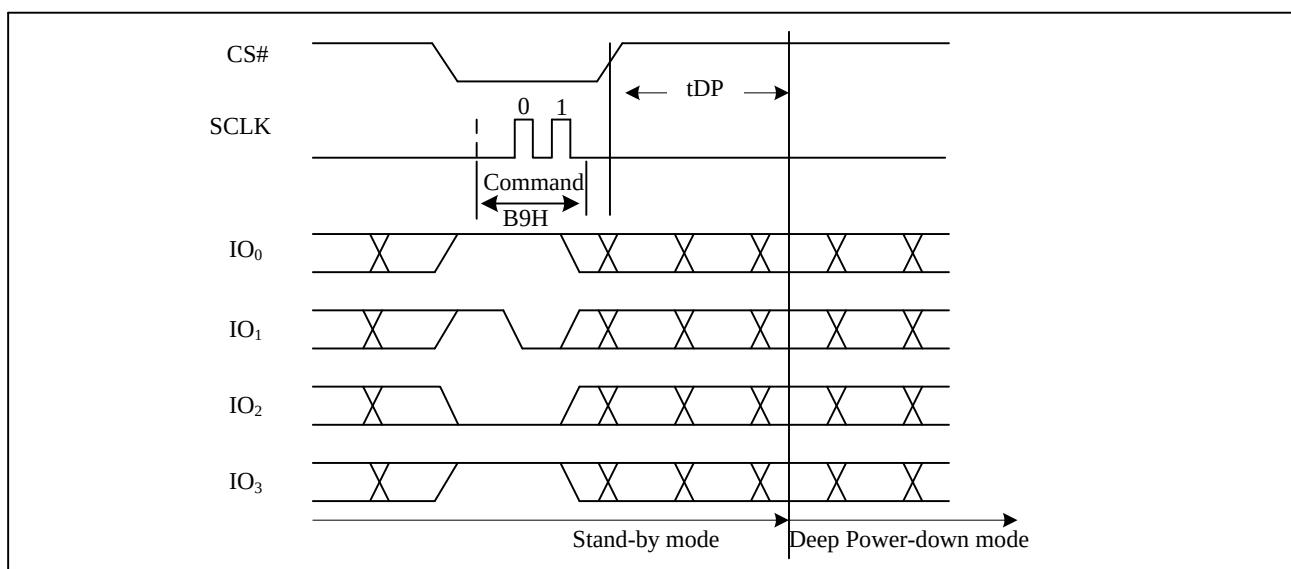
Figure21a. Deep Power-Down Sequence Diagram (QPI)
