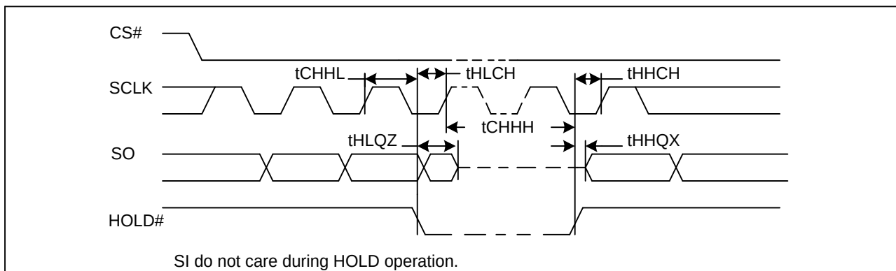
Figure44. Hold Timing
