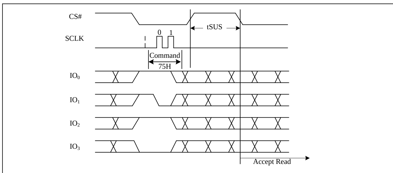
Figure28a. Program/Erase Suspend Sequence Diagram (QPI)
