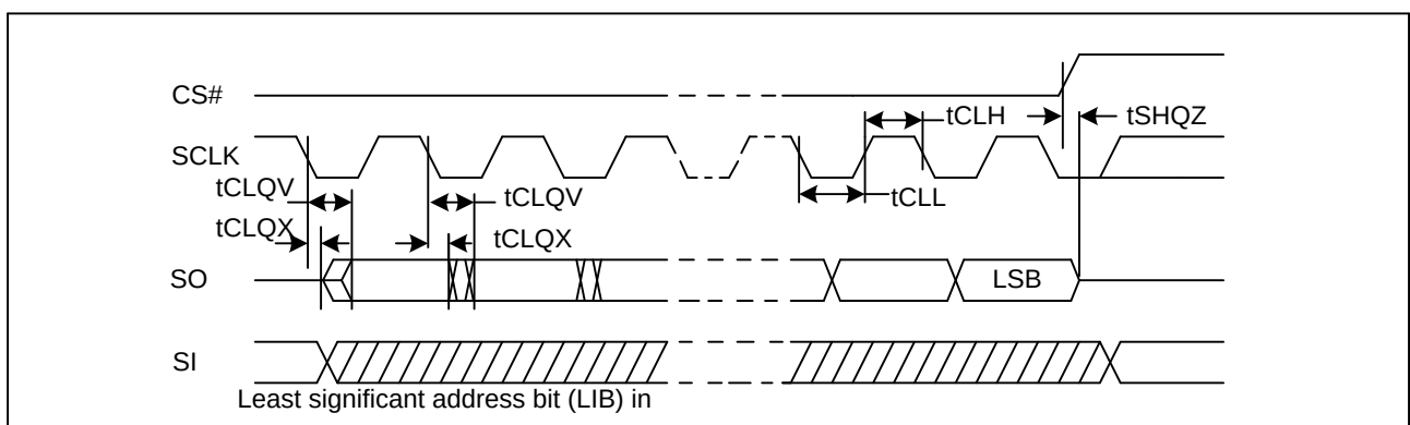
Figure43. Output Timing
