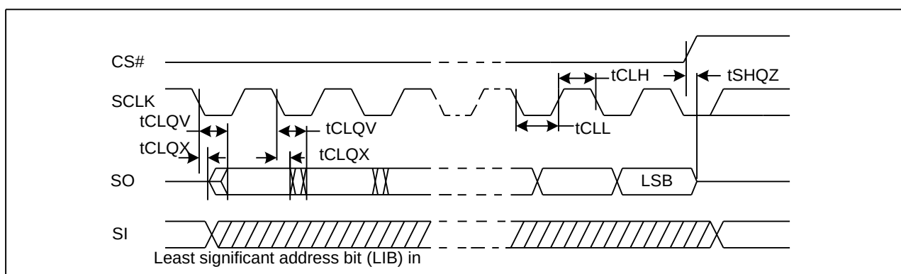
Figure 39. Output Timing
