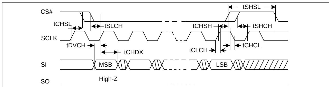
Figure 38. Serial Input Timing
