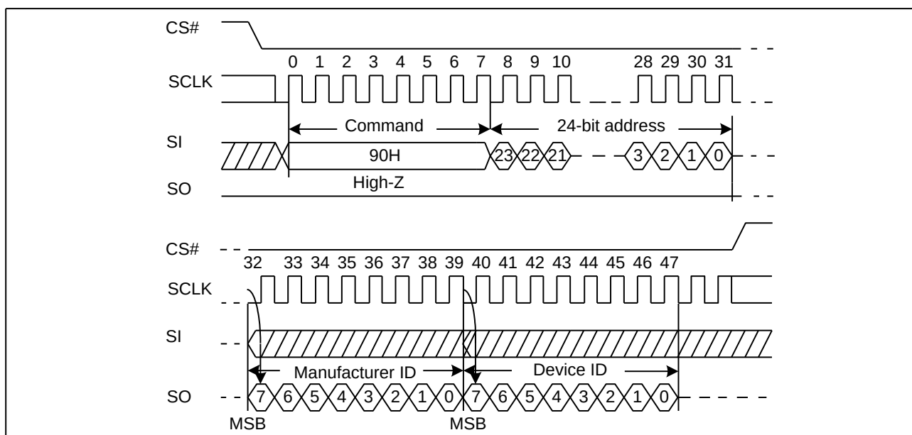
Figure27. Read Manufacturer ID/ Device ID Sequence Diagram
