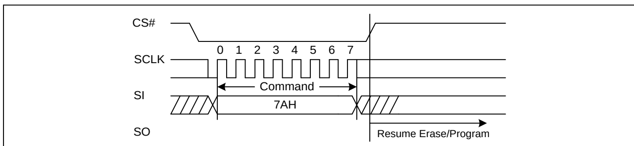
Figure32. Program/Erase Resume Sequence Diagram
