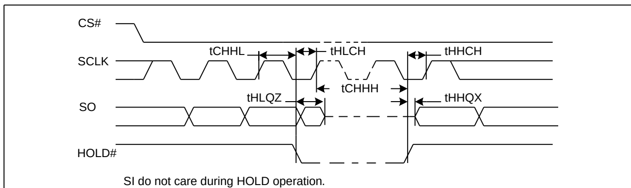
Figure45. Hold Timing
