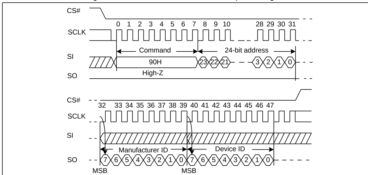
Figure26. Read Manufacturer ID/ Device ID Sequence Diagram
