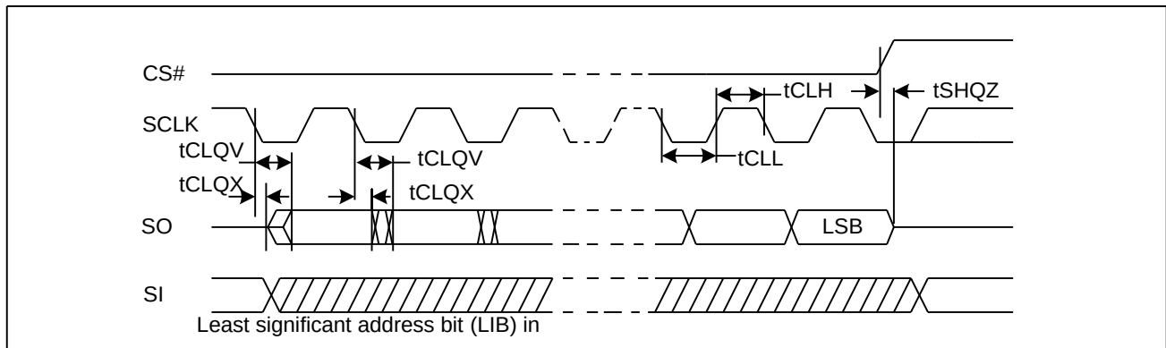
Figure42. Output Timing
