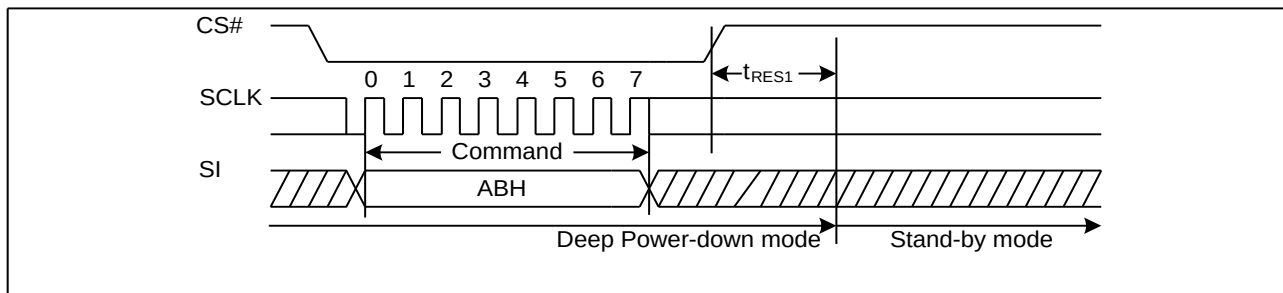
Figure25. Release Power-Down/Read Device ID Sequence Diagram
