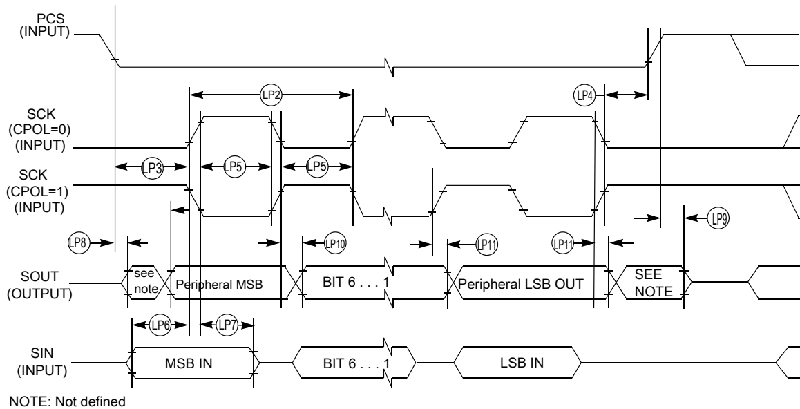
Figure 40. LPSPI Peripheral mode timing (CPHA = 0)
