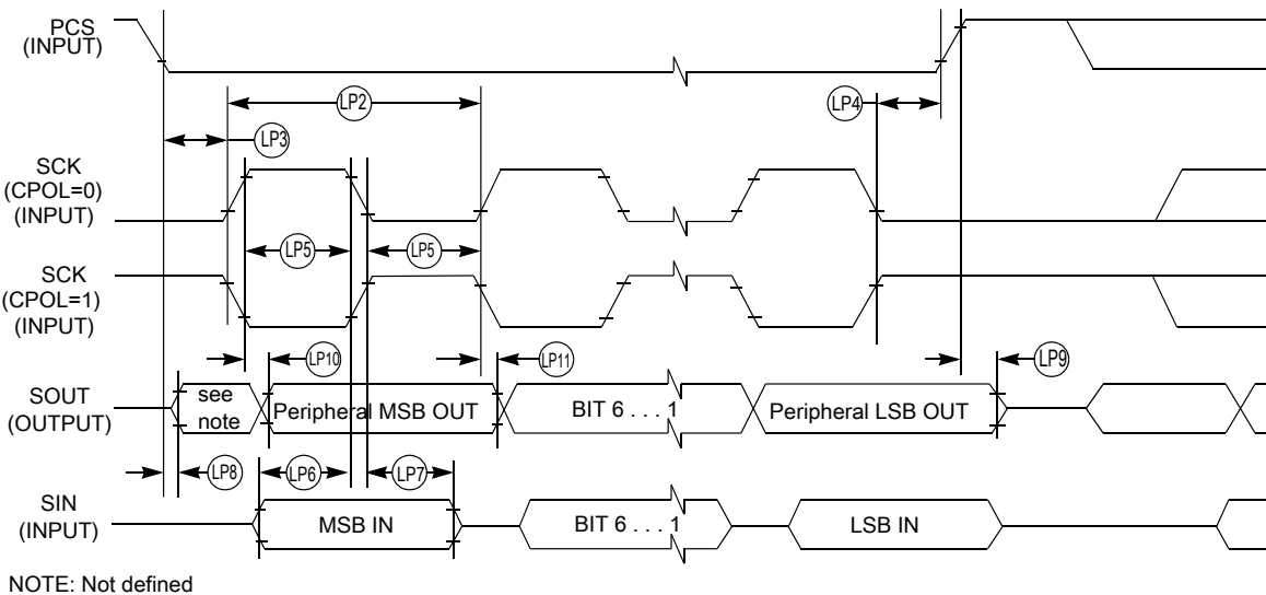
Figure 41. LPSPI Peripheral mode timing (CPHA = 1)
