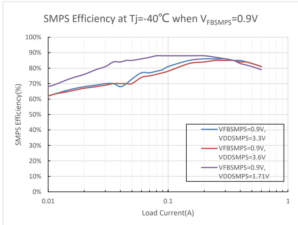
Figure 4-6. Typical SMPS efficiency (%) vs load current(A) in Run mode at T_J = -40^\circ C when V_{FBSMPS} = 0.9V
