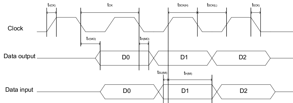
Figure 4-15. OSPI timing diagram - DTR mode
