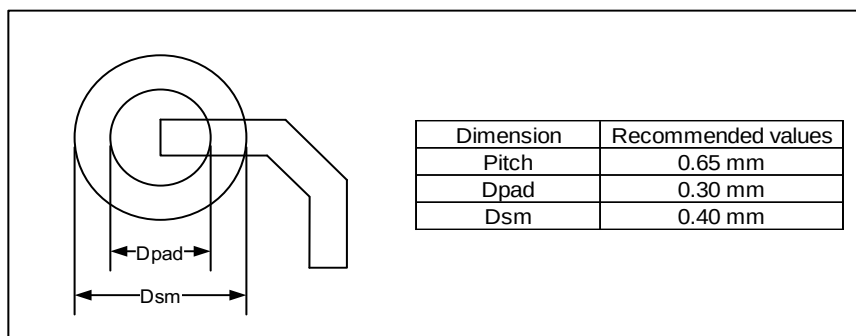
Figure 5-2. BGA176 recommended footprint
