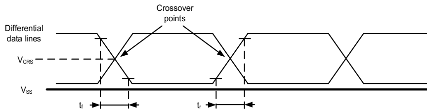
Figure 4-18. USBFS timings: definition of data signal rise and fall time
