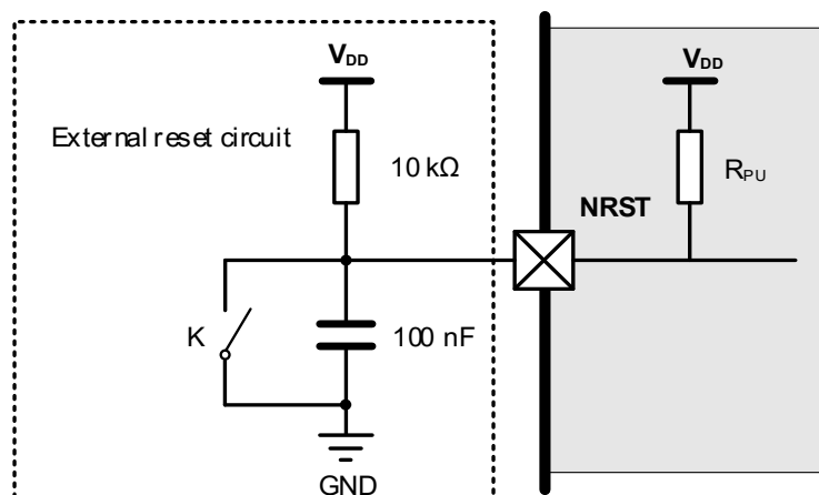
Figure 4-10. Recommended external NRST pin circuit
