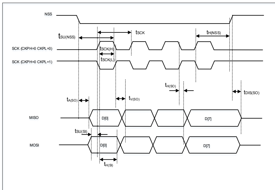
Figure 4-13. SPI timing diagram - slave mode
