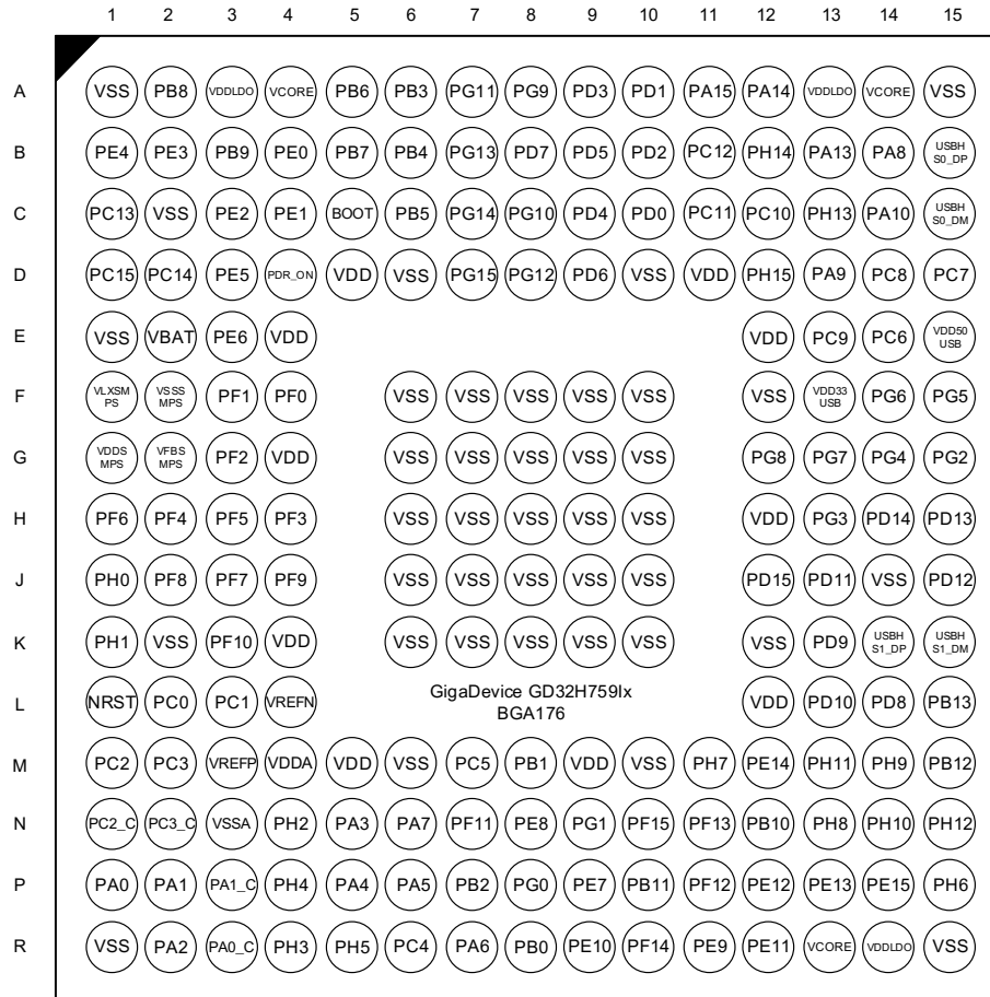
Figure 2-2. GD32H759Ix BGA176 pinouts
