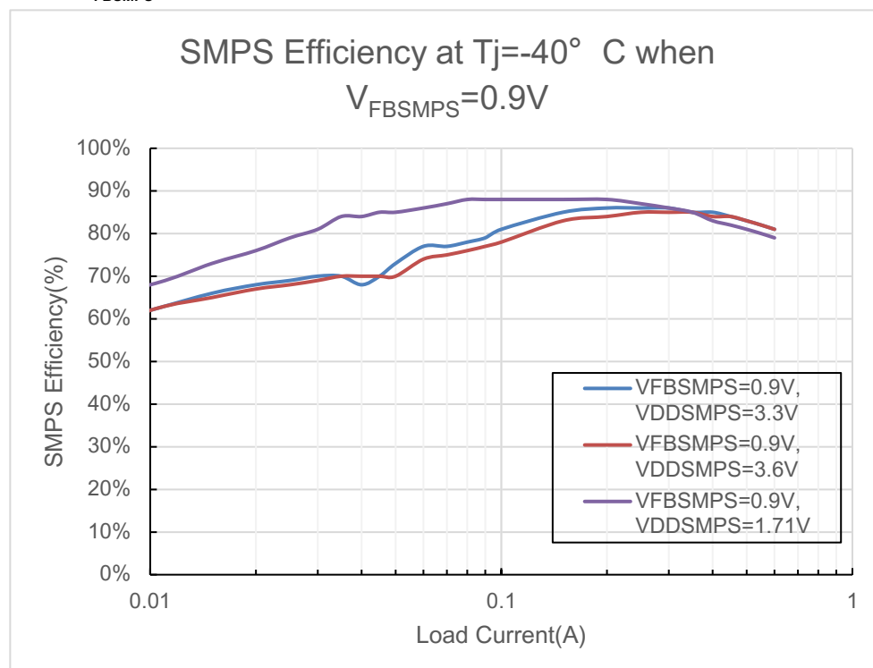
Figure 4-6. Typical SMPS efficiency (%) vs load current(A) in Run mode at T_J = -40^\circ\text{C} when V_{FBSMPS} = 0.9\text{V}
