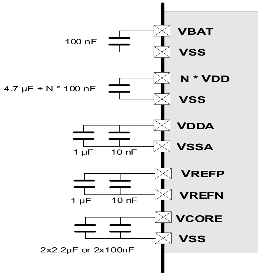
Figure 4-2. Recommended power supply decoupling capacitors (1)(2)(3)
