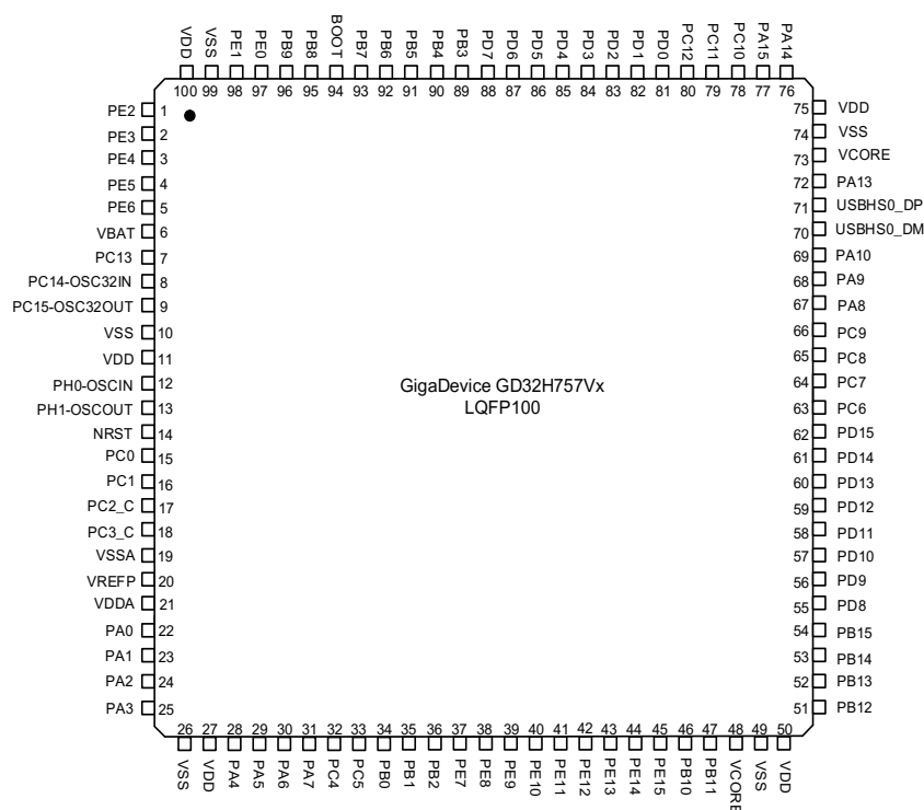
Figure 2-4. GD32H757Vx LQFP100 pinouts
