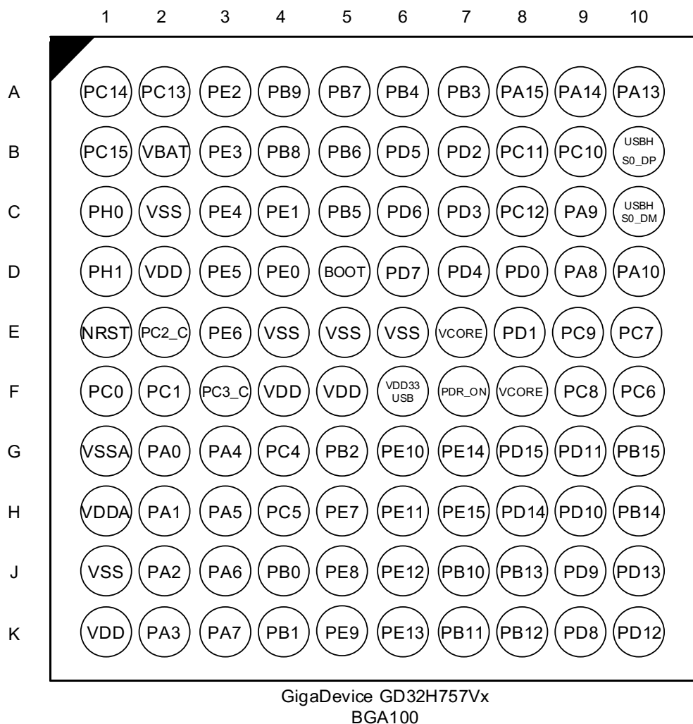
Figure 2-2. GD32H757Vx BGA100 pinouts
