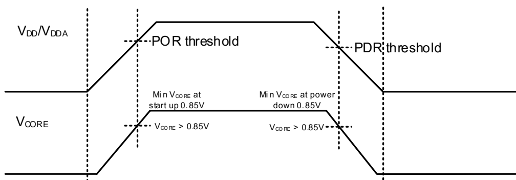
Figure 4-1. Bypass Mode Power-up and Power-down Timing Diagram (1)(2)(3)
