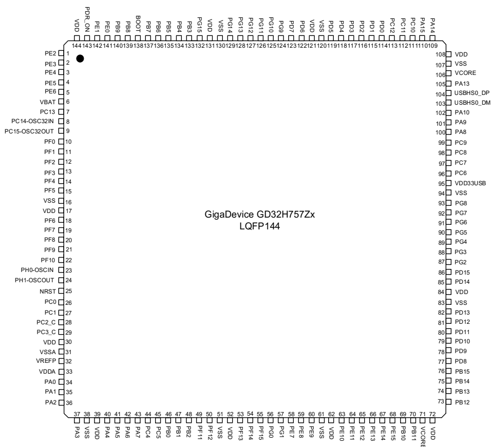
Figure 2-3. GD32H757Zx LQFP144 pinouts
