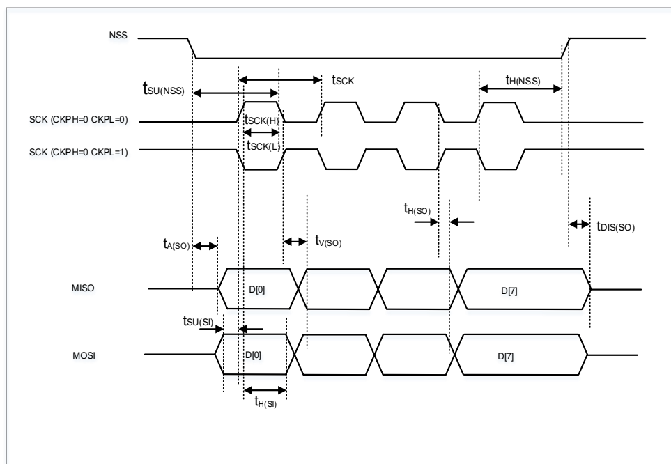
Figure 4-9. SPI timing diagram - slave mode
