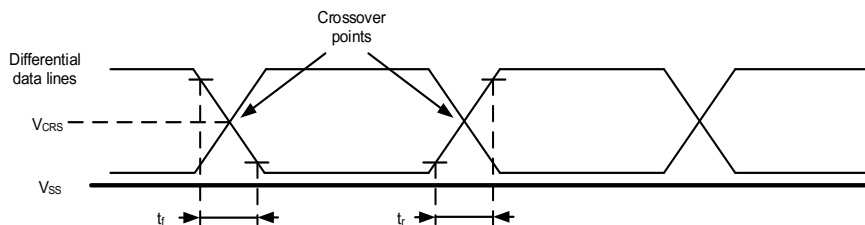
Figure 4-14. USBFS timings: definition of data signal rise and fall time
