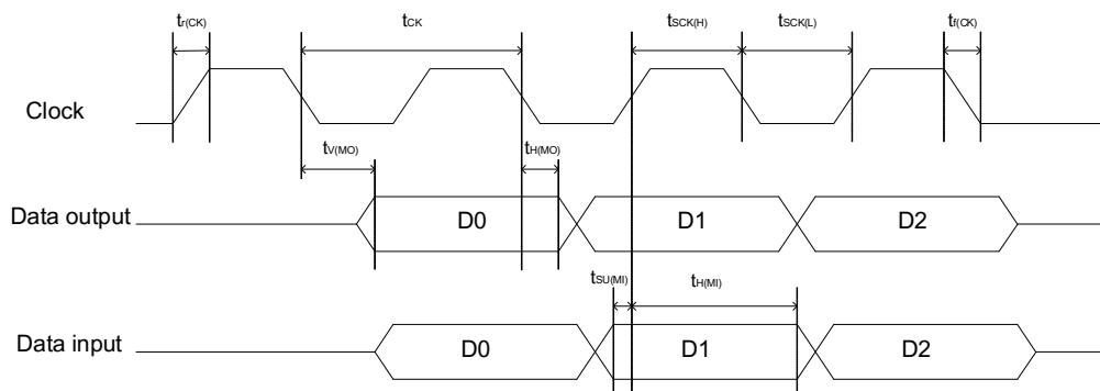
Figure 4-11. OSPI timing diagram - DTR mode
