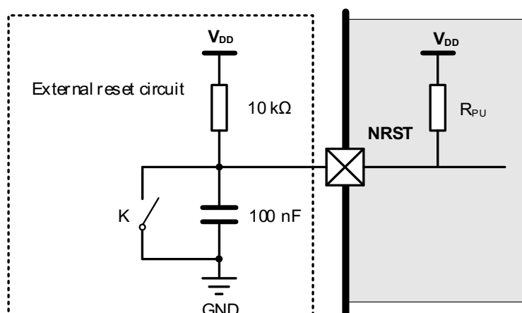
Figure 4-6. Recommended external NRST pin circuit
