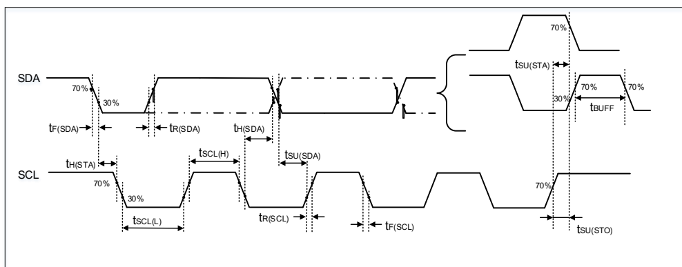
Figure 4-7. I2C bus timing diagram
