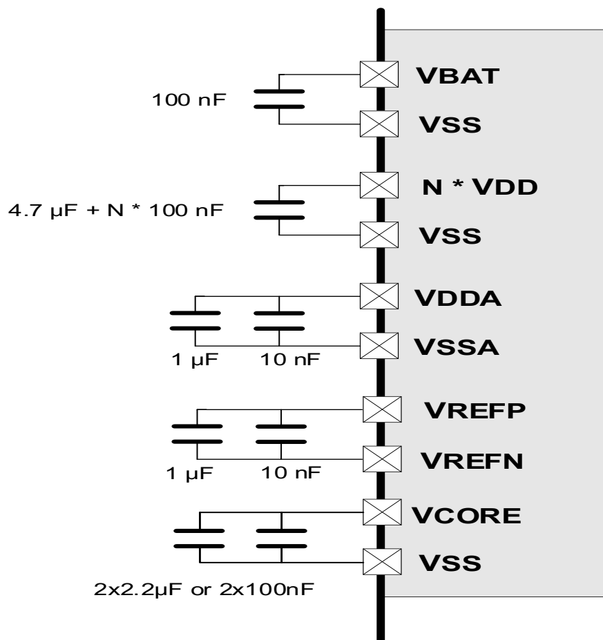
Figure 4-2. Recommended power supply decoupling capacitors (1)(2)(3)
