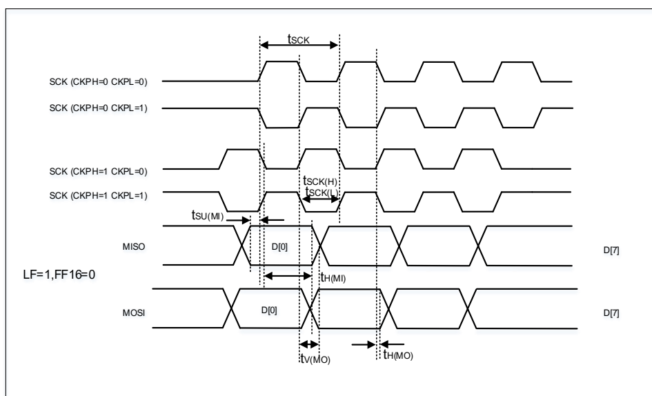
Figure 4-8. SPI timing diagram - master mode
