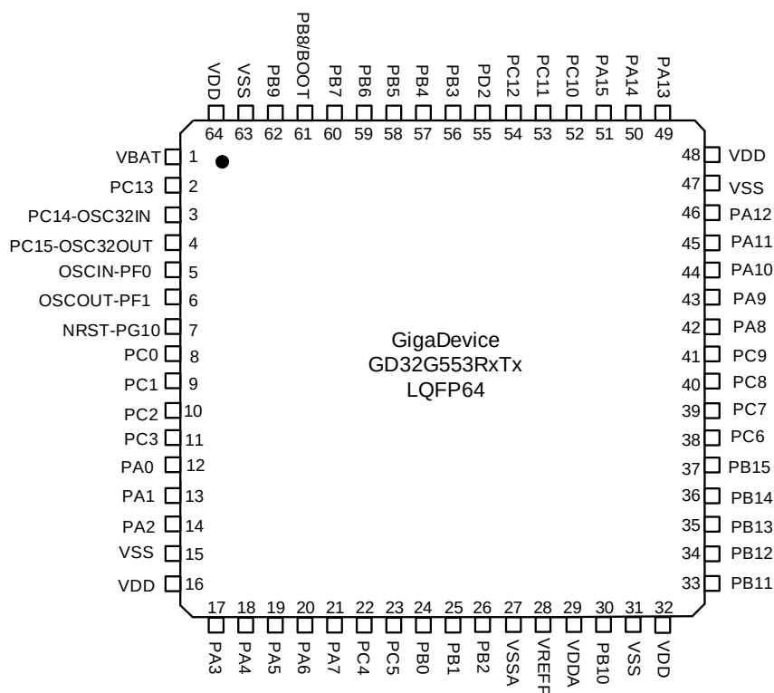
Figure 2-6. GD32G553RxTx LQFP64 pinouts (1)
