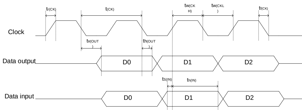
Figure 4-15. QSPI timing diagram - SDR mode
