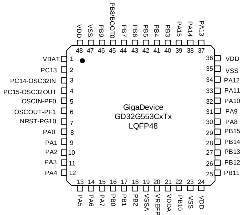
Figure 2-7. GD32G553CxTx LQFP48 pinouts (1)
