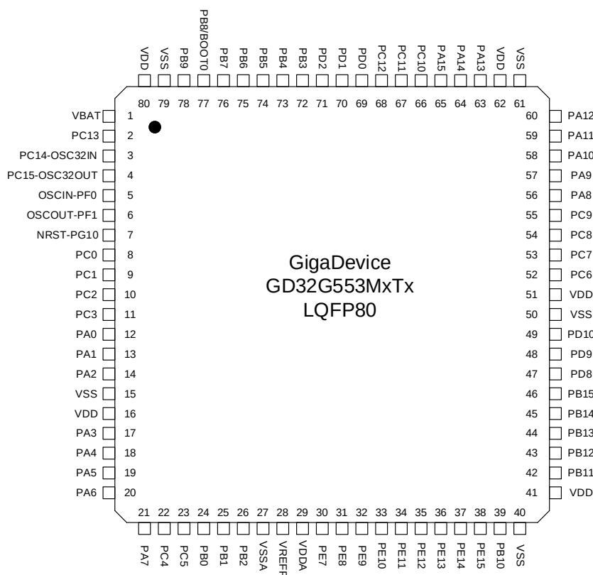
Figure 2-5. GD32G553MxTx LQFP80 pinouts (1)
