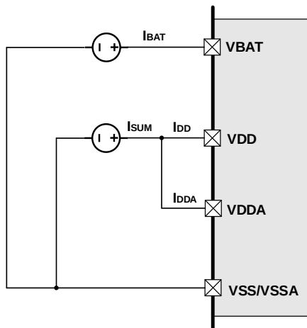
Figure 4-2. Power consumption measurement diagram
