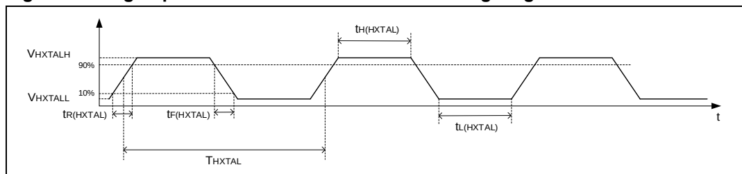
Figure 4-4. High-speed external clock source AC timing diagram
