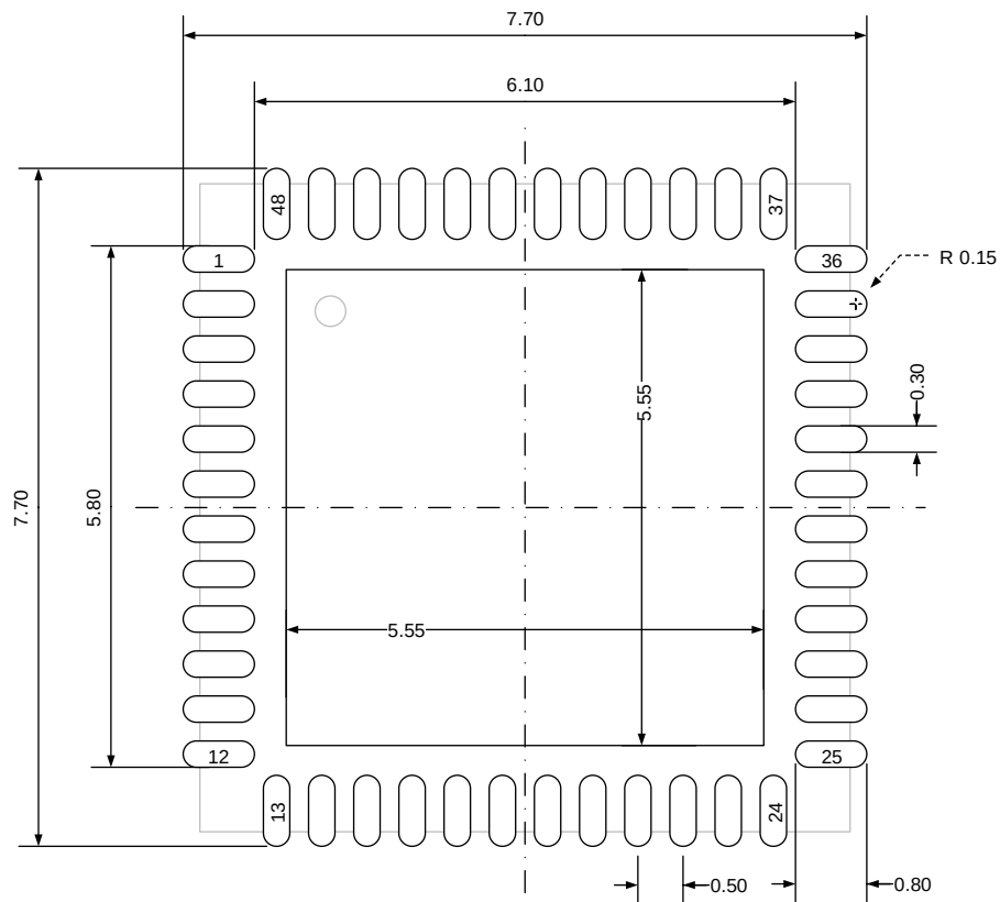
Figure 5-14. QFN48 recommended footprint
