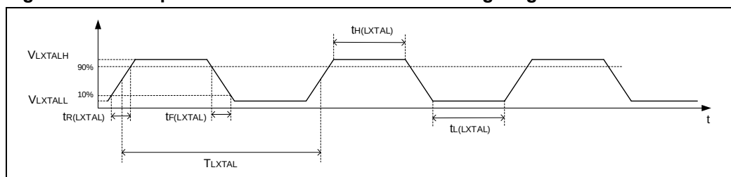
Figure 4-5. Low-speed external clock source AC timing diagram
