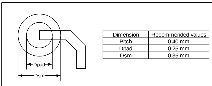
Figure 5-6. WLCSP81 recommended footprint
