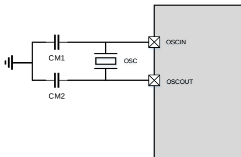
Figure 4-6. Recommended external OSCIN and OSCOUT pins circuit for crystal
