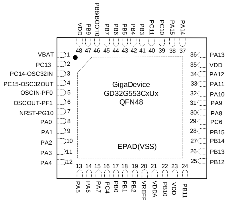
Figure 2-8. GD32G553CxUx QFN48 pinouts (1)(2)
