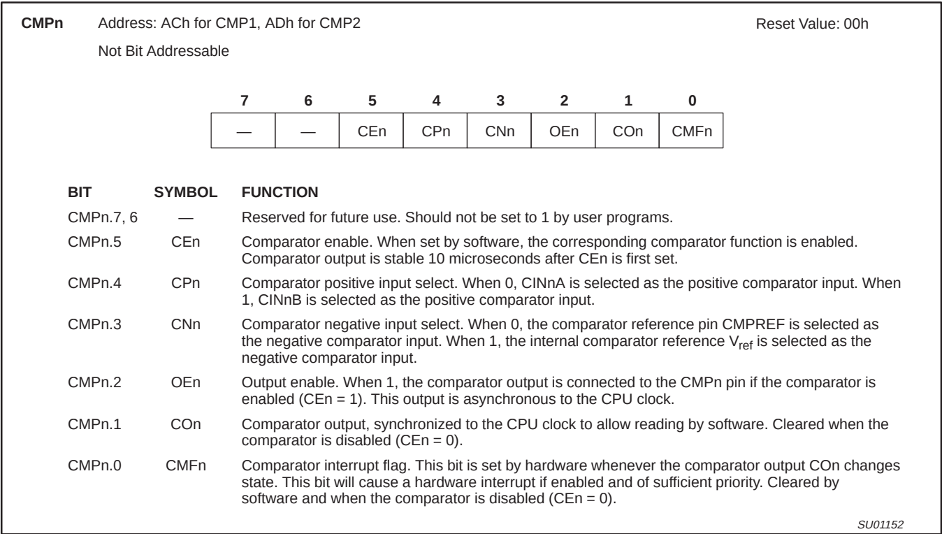
Figure 4. Comparator Control Registers (CMP1 and CMP2)
