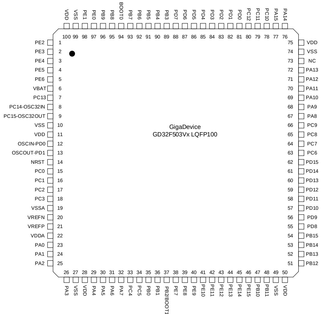
Figure 2-2. GD32F503Vx LQFP100 pinouts
