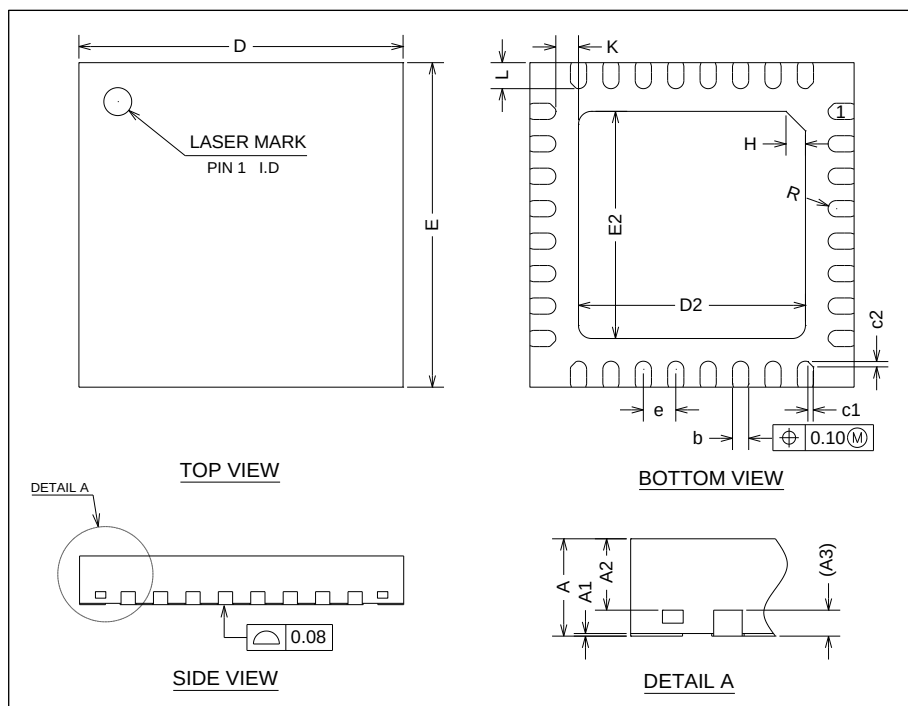
Figure 5-13. QFN32 package outline
