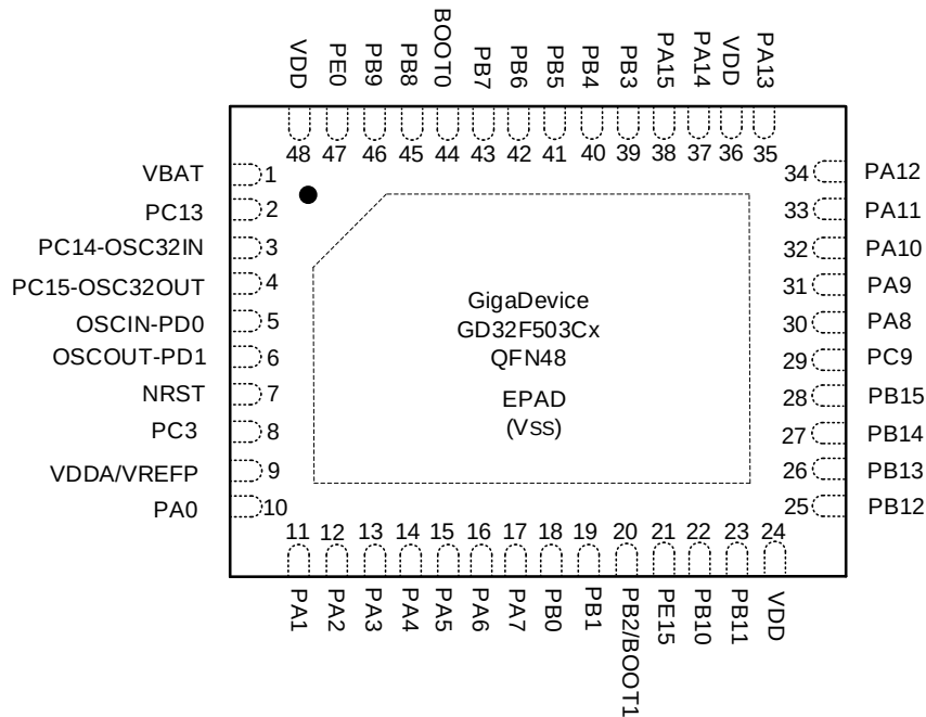
Figure 2-7. GD32F503Cx QFN48 pinouts
