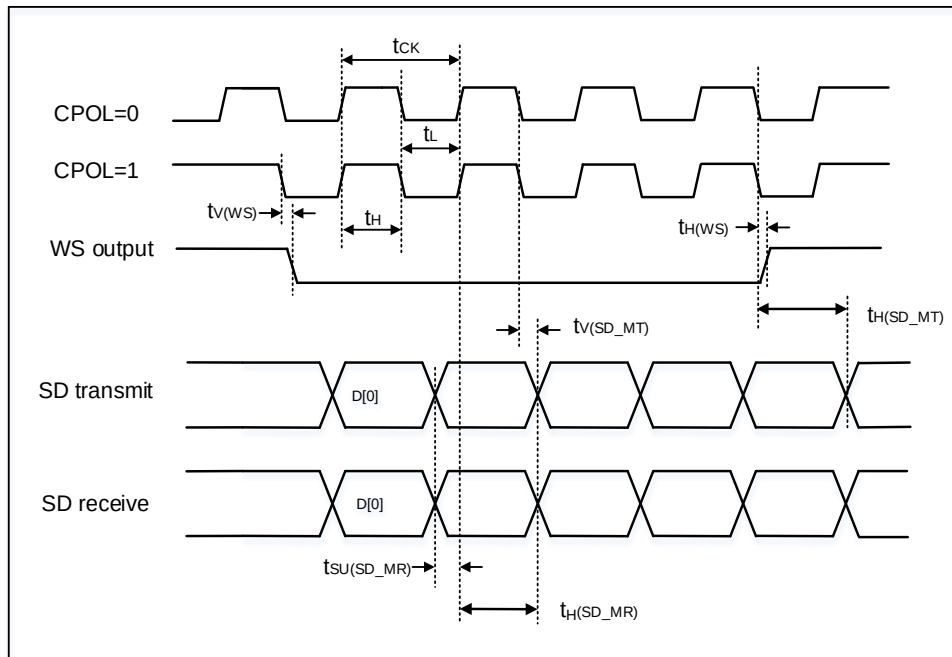
Figure 4-17. I2S timing diagram - master mode
