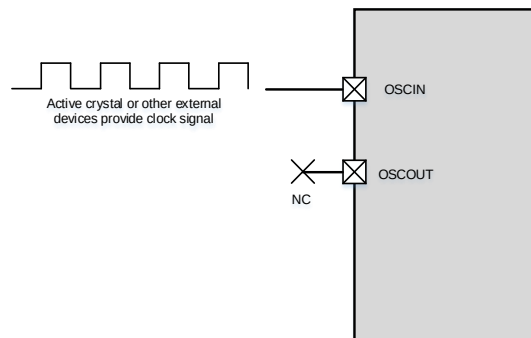
Figure 4-8. Recommended external OSCIN and OSCOUT pins circuit for oscillator
