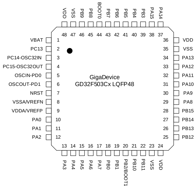
Figure 2-6. GD32F503Cx LQFP48 pinouts
