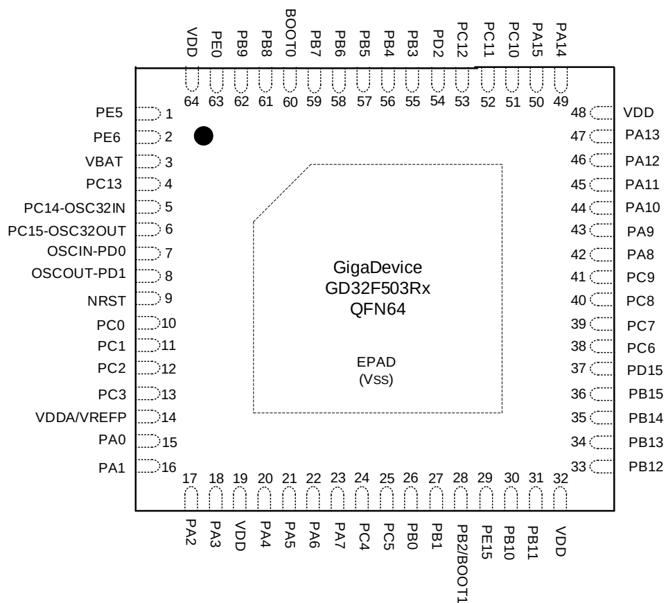
Figure 2-4. GD32F503Rx QFN64 pinouts
