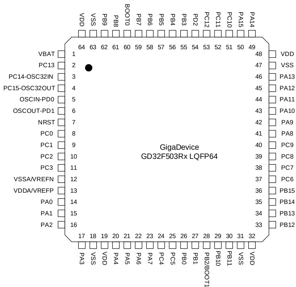
Figure 2-3. GD32F503Rx LQFP64 pinouts
