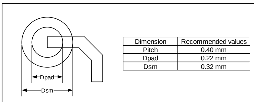
Figure 5-8. BGA64 recommended footprint
