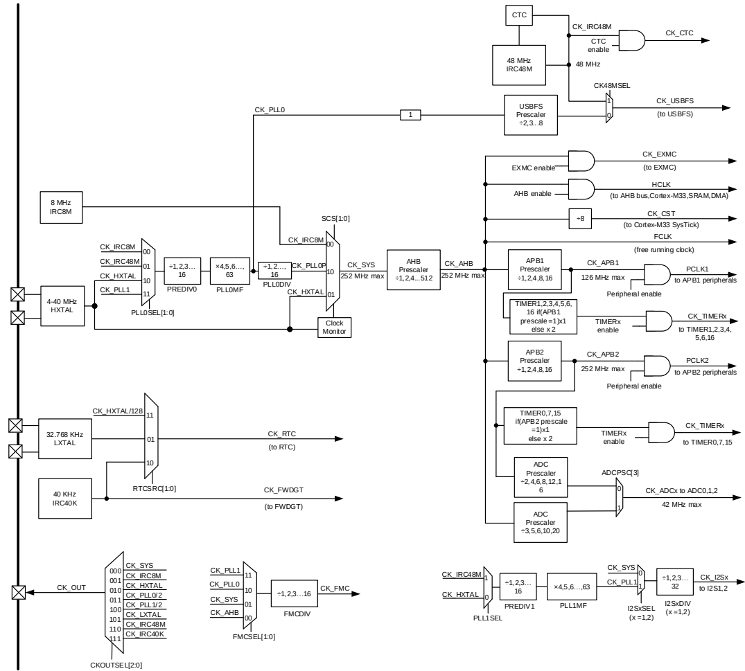
Figure 2-9. GD32F503xx clock tree
