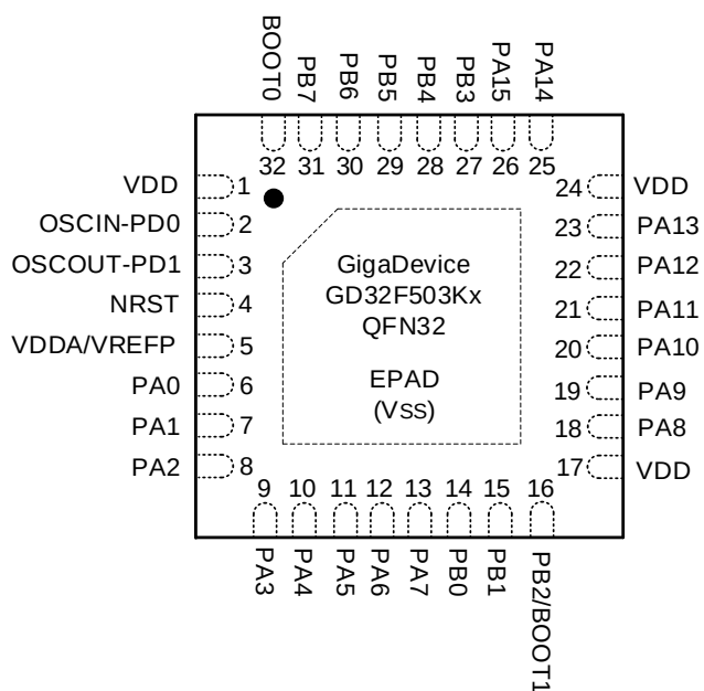
Figure 2-8. GD32F503Kx QFN32 pinouts
