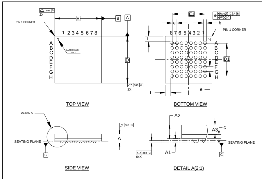
Figure 5-7. BGA64 package outline
