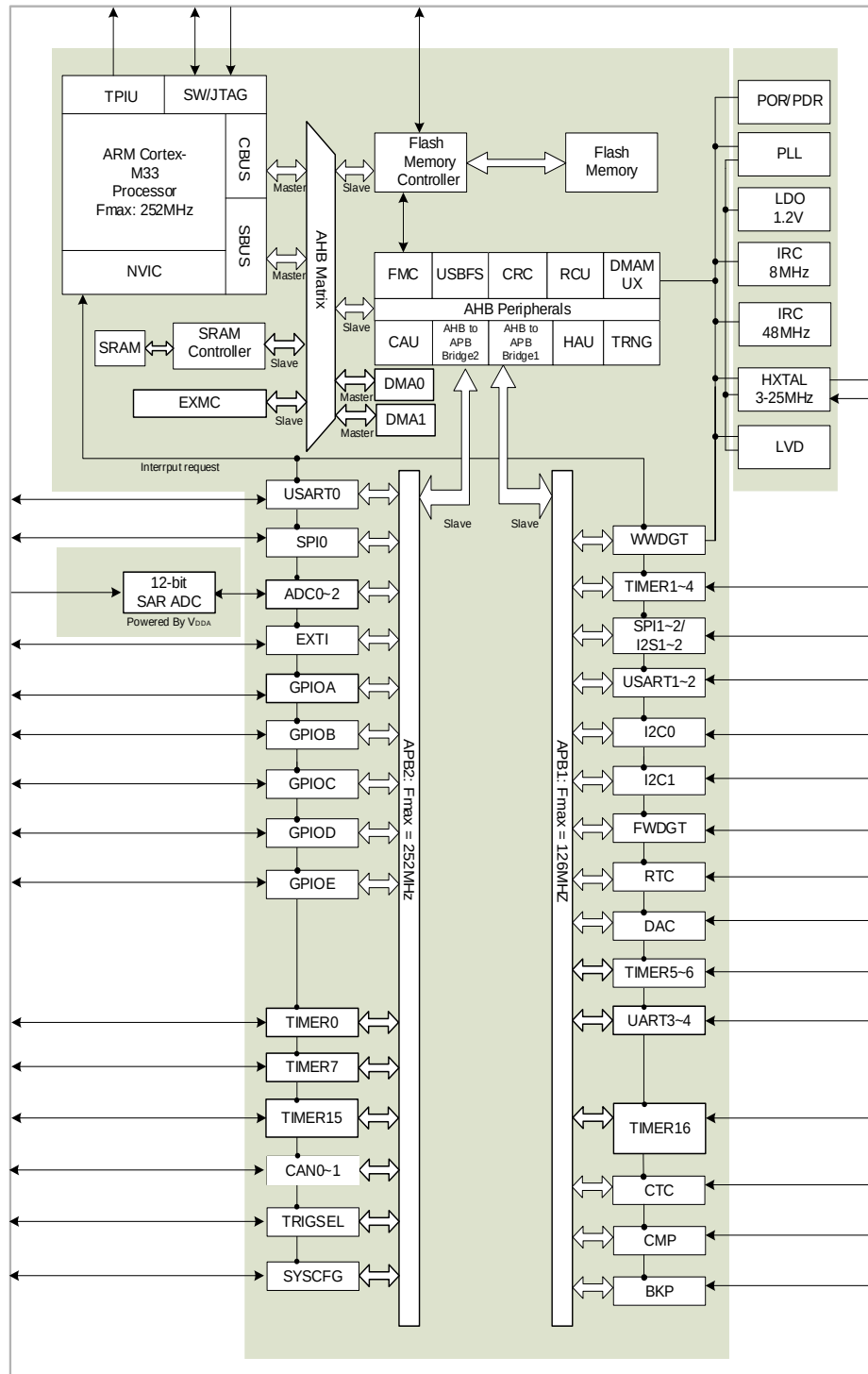
Figure 2-1. GD32F503xx block diagram
