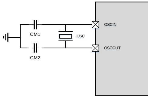
Figure 4-7. Recommended external OSCIN and OSCOUT pins circuit for crystal
