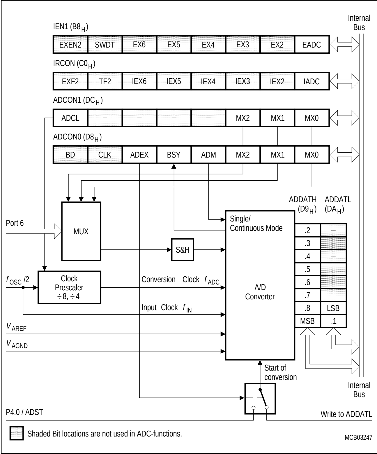
Figure 14 A/D Converter Block Diagram
