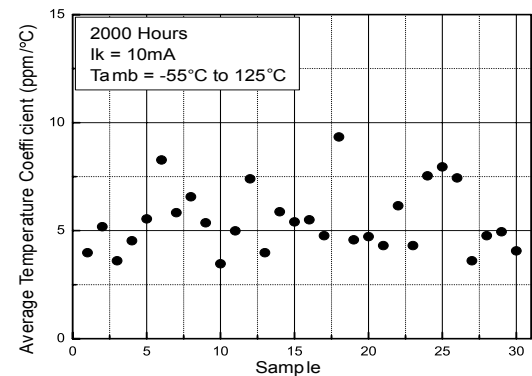
Figure 58. Average temperature coefficient at 2000 hrs, I_k = 10 mA
