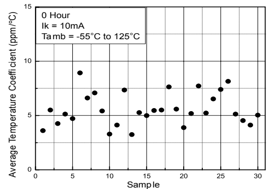
Figure 56. Average temperature coefficient at 0 hr, I_k = 10 mA
