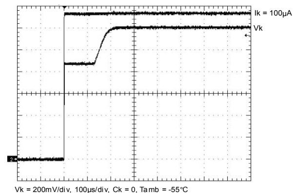
Figure 30. Cathode current step resp. at -55 °C, C_k = 0 , \Delta I_k = 100 \mu A
