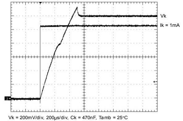
Figure 38. Cathode current step resp. at 25 °C, C_k = 470 \text{ nF} , \Delta I_k = 1 \text{ mA}
