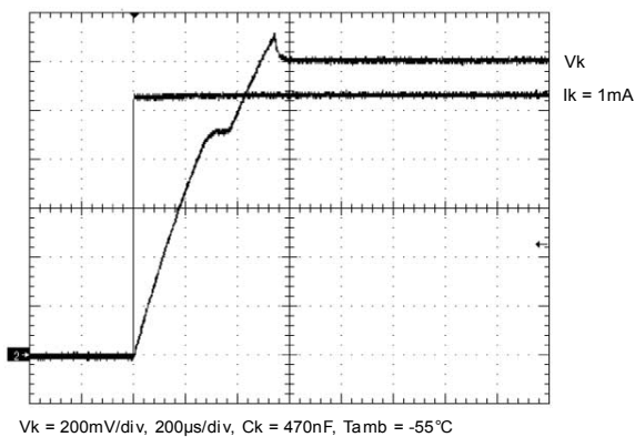
Figure 39. Cathode current step resp. at -55 °C, C_k = 470 \text{ nF} , \Delta I_k = 1 \text{ mA}
