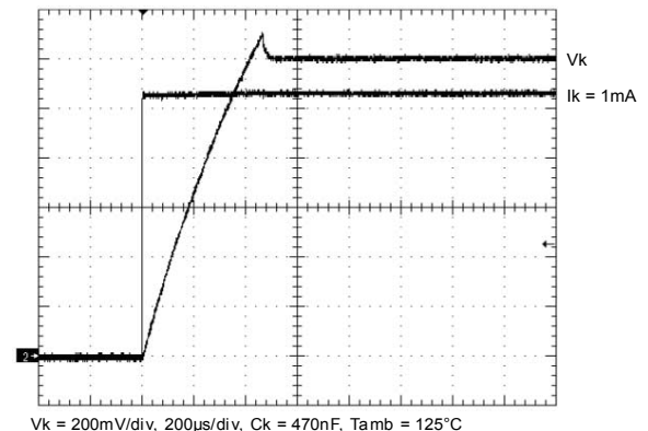
Figure 40. Cathode current step resp. at 125 °C, C_k = 470 \text{ nF} , \Delta I_k = 1 \text{ mA}
