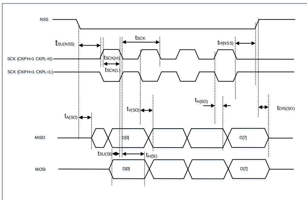
Figure 4-10. SPI timing diagram - slave mode(CKPH=1)
