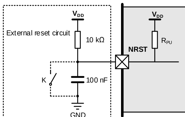
Figure 4-6. Recommended external NRST pin circuit (1)
