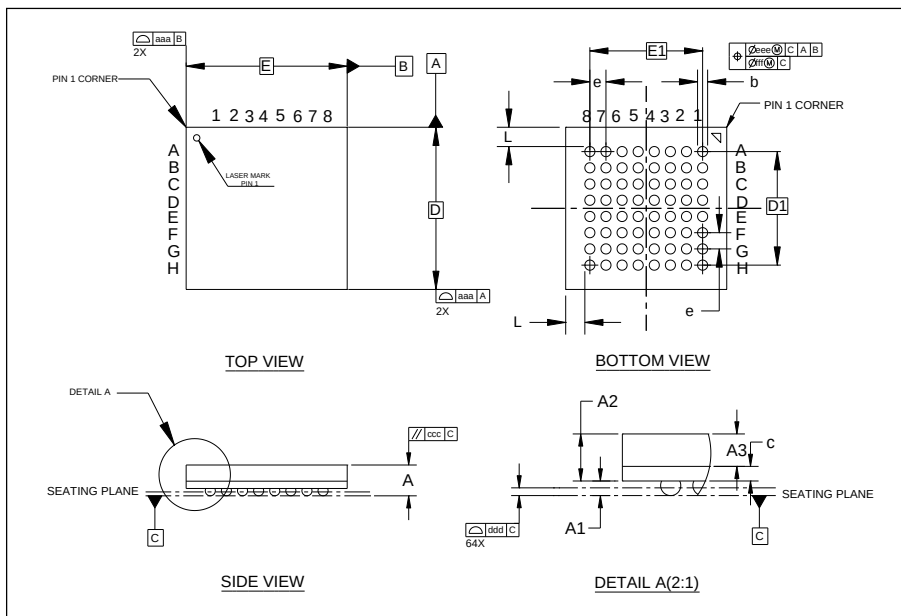
Figure 5-1. BGA64(4x4) package outline
