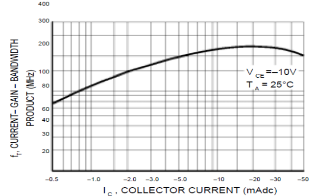
Figure 6. Current-Gain-Bandwidth Product
