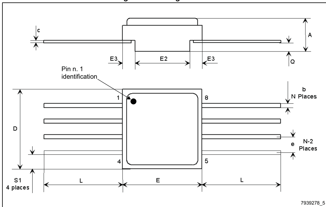
Figure 2. Package outline
